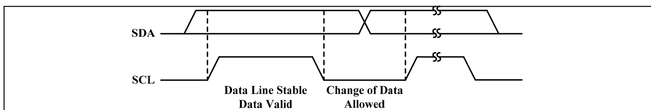
Figure 3 Bit Transfer
