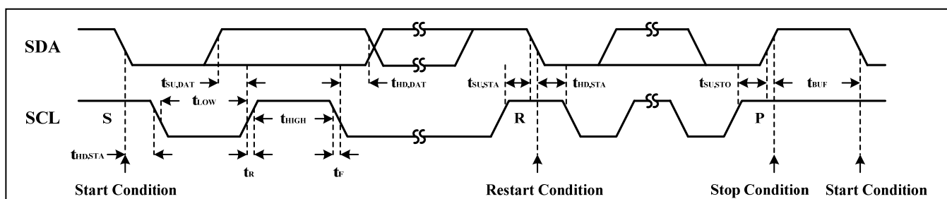
Figure 2 Interface Timing
