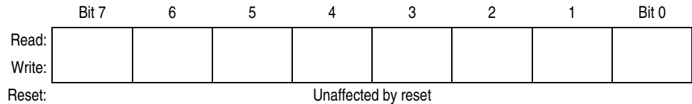
Figure 9-2. Accumulator (A)
