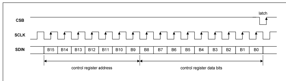
Figure 51 3-Wire Serial Control Interface
