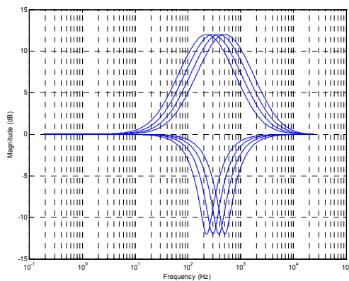
Figure 67 EQ Band 2 – Peak Filter Centre Frequencies, EQ2BW=0
