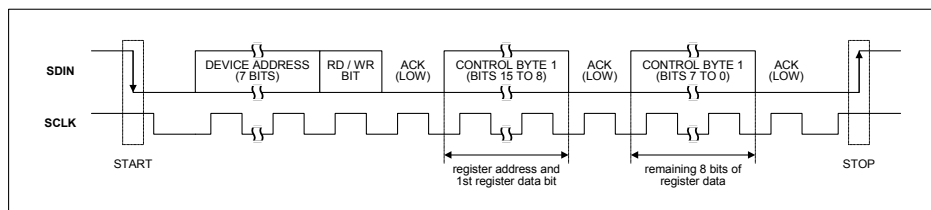
Figure 52 2-Wire Serial Control Interface
