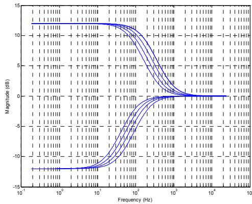
Figure 65 EQ Band 1 Low Frequency Shelf Filter Cut-offs
