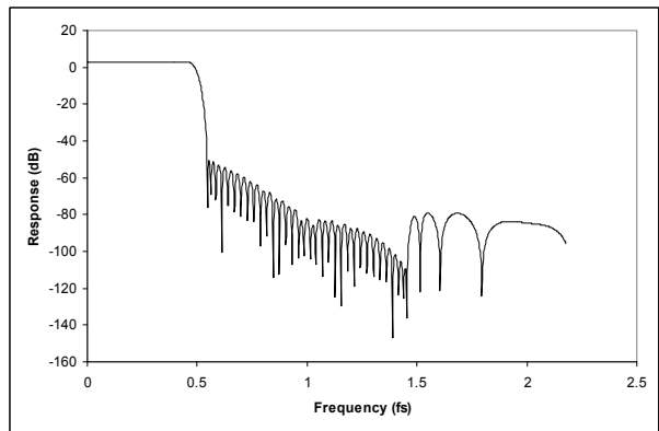
Figure 57 DAC Digital Filter Frequency Response (64xOSR)
