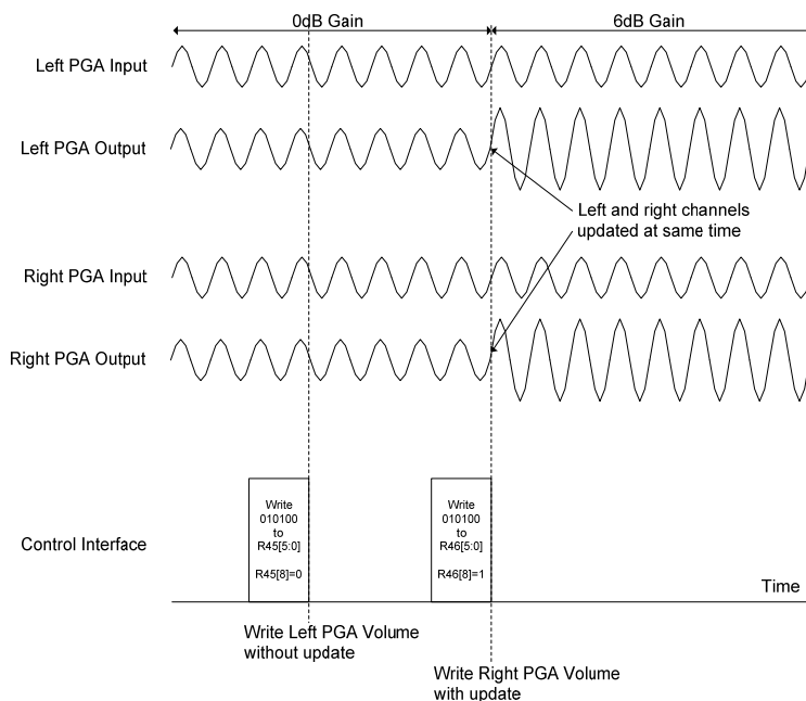
Figure 10 Simultaneous Left and Right Volume Updates
