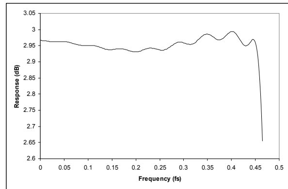
Figure 58 DAC Digital Filter Ripple (64xOSR)
