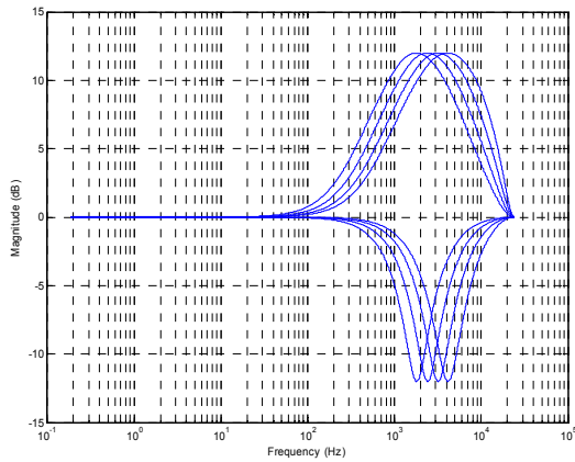
Figure 73 EQ Band 4 – Peak Filter Centre Frequencies, EQ3f Figure 74 EQ Band 4 – Peak Filter Gains for Lowest Cut-off Frequency, EQ4BW=0
