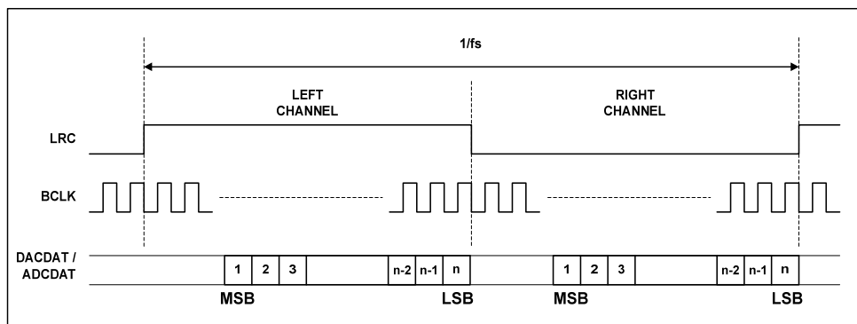
Figure 44 Right Justified Audio Interface (assuming n-bit word length)
