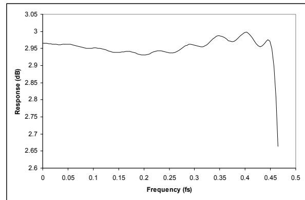
Figure 56 DAC Digital Filter Ripple (128xOSR)
