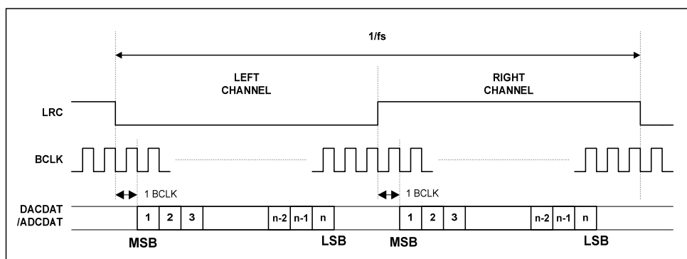
Figure 45 I^2S Audio Interface (assuming n-bit word length)
