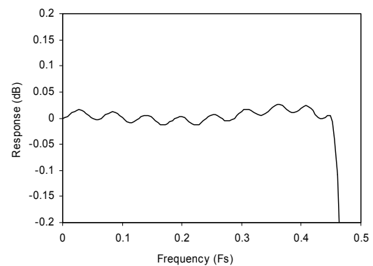
Figure 60 ADC Digital Filter Ripple
