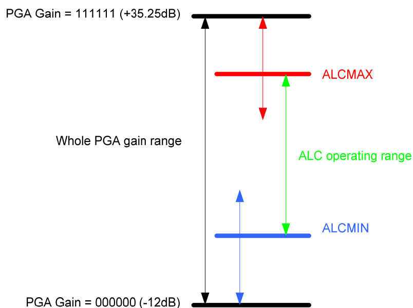
Figure 19 ALC Min/Max Gain
