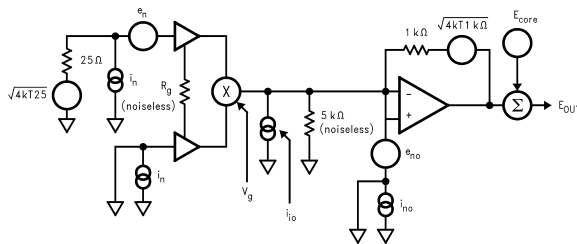
FIGURE 7. Noise Model for Typical Circuit
