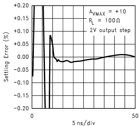
Settling Time, V_g = 2\text{V}
