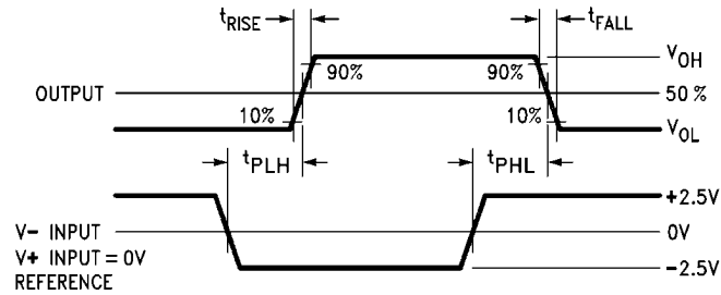
FIGURE 2. Propagation Delay
