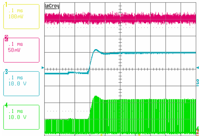
FIGURE 30. V_{IN} TRANSIENT TEST, V_{IN} = 8 \rightarrow 19V , I_O = 2A , V_{ID} = 1.1V , Ch1: V_O , Ch2: V_O , Ch3: V_{IN} , Ch4: PHASE
