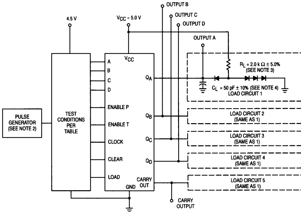
TEST CIRCUIT
