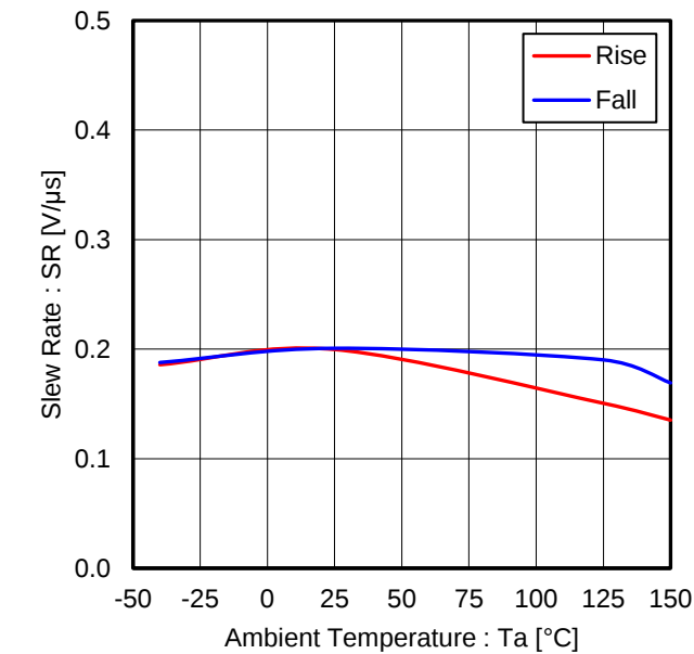
Figure 25. Slew Rate vs Ambient Temperature (V CC = 5 V, R L = 2 kΩ)
