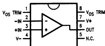
Dual-In-Line Package
