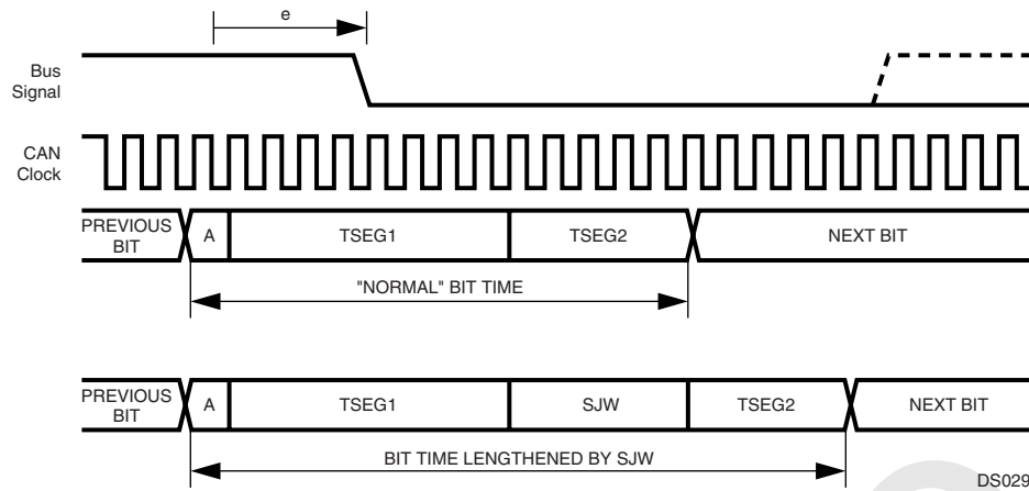
Figure 36. Resynchronization ( e > SJW )
