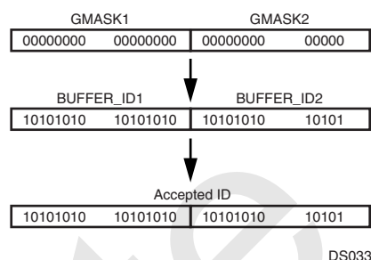
Figure 40. Acceptance of a Single Identifier
