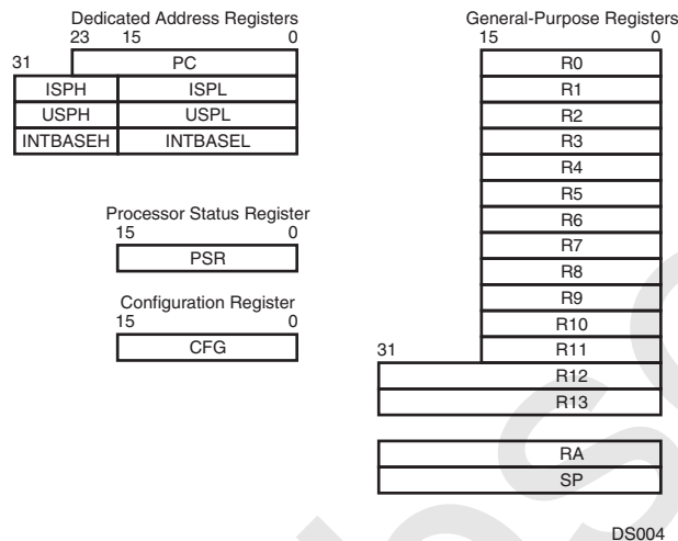
Figure 1. CPU Registers
