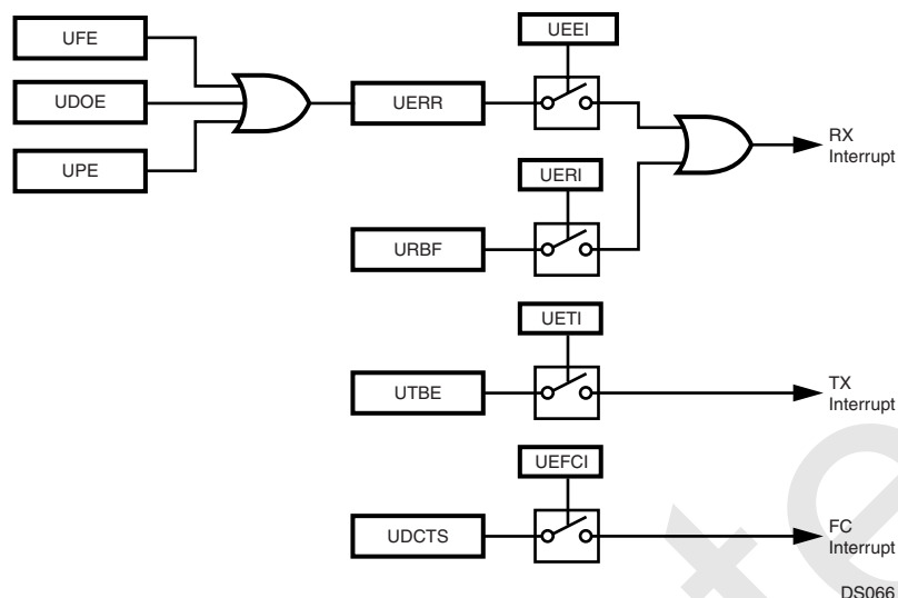
Figure 73. UART Interrupts
