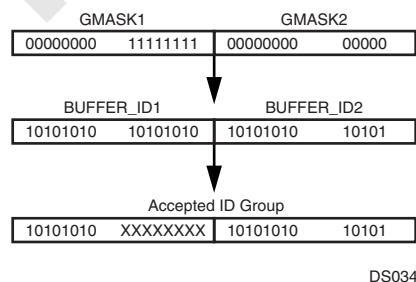
Figure 41. Acceptance of a Group of Identifiers
