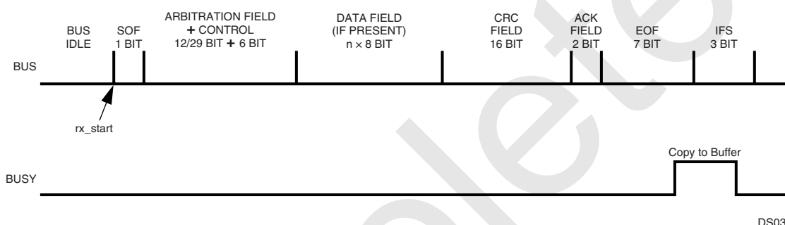
Figure 44. Receive Timing
