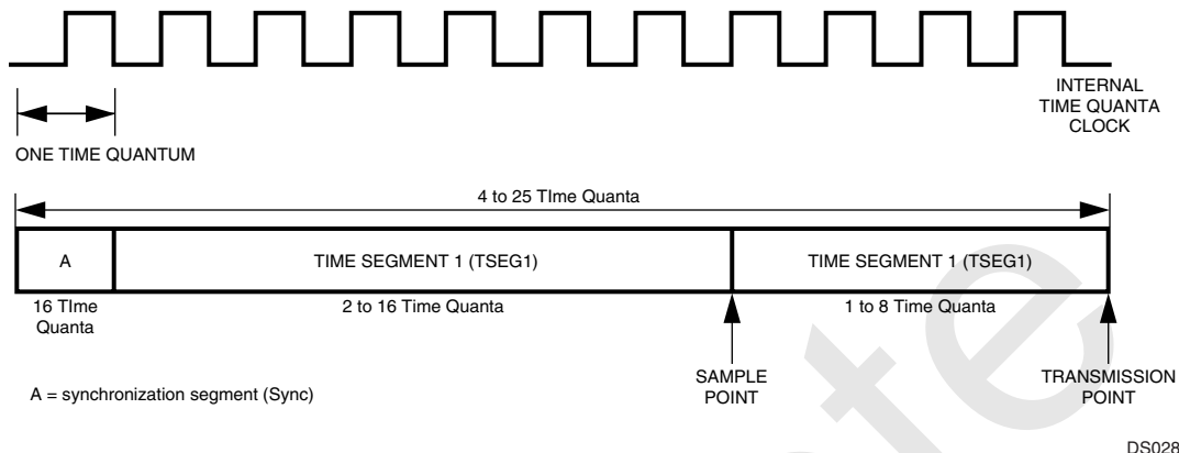
Figure 35. Bit Timing
