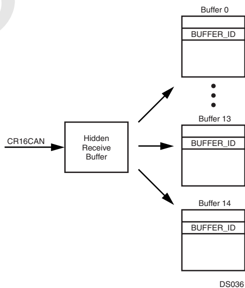
Figure 43. Receive Buffer
