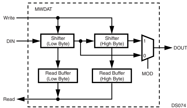
Figure 81. MWDAT Register
