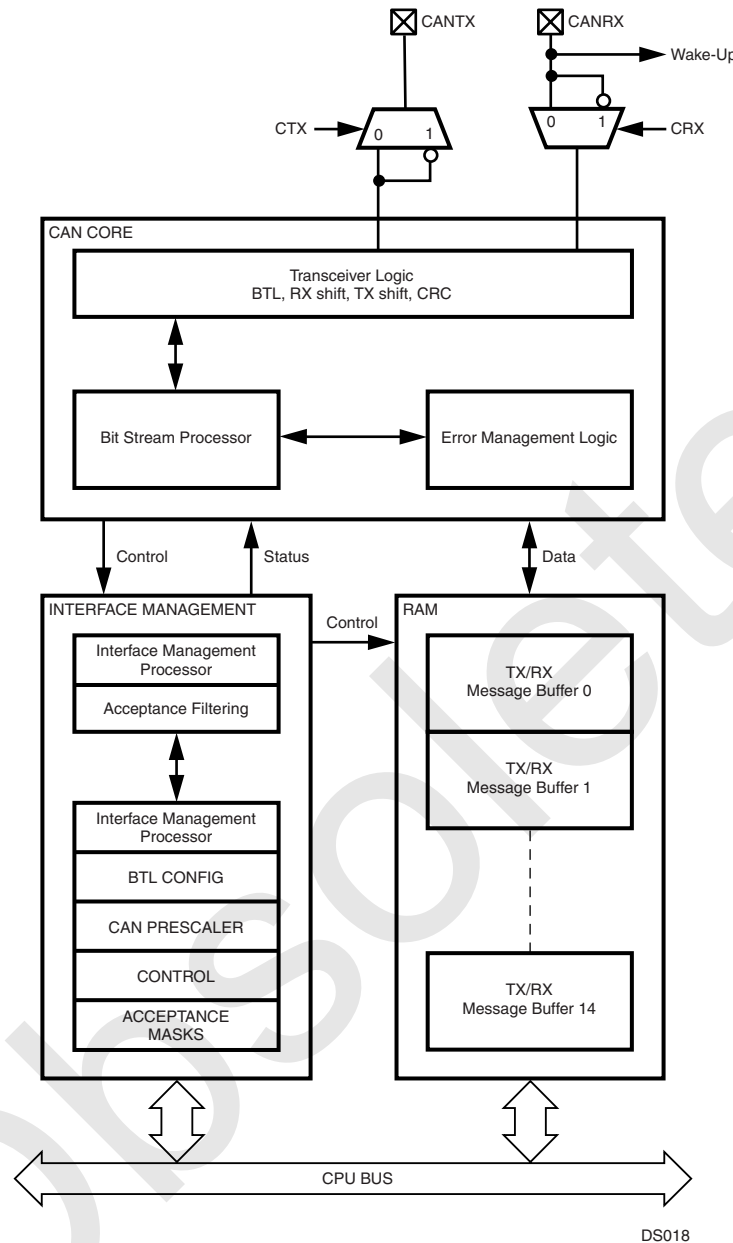
Figure 25. CAN Block Diagram
