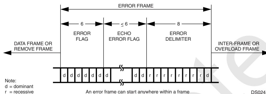
Figure 31. Error Frame
