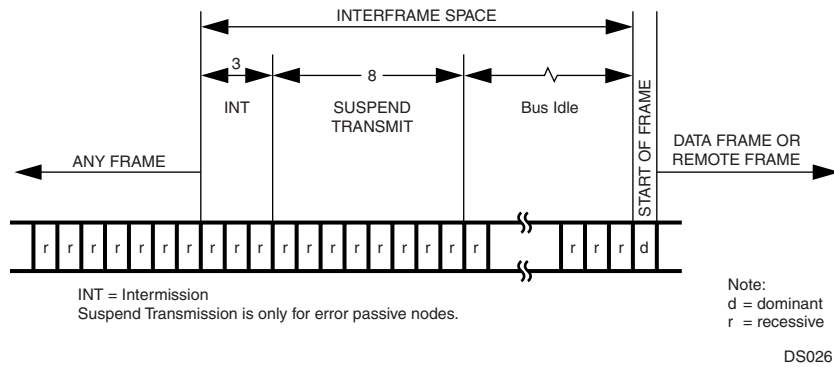
Figure 33. Interframe Space
