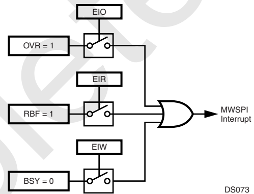
Figure 80. MWSPI Interrupts
