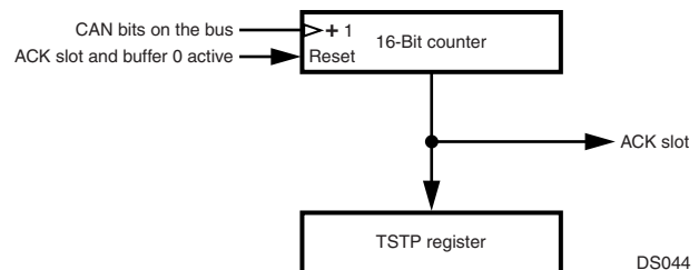
Figure 51. Time Stamp Counter
