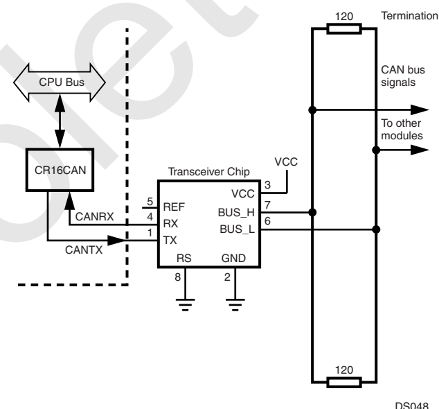
Figure 55. External Transceiver
