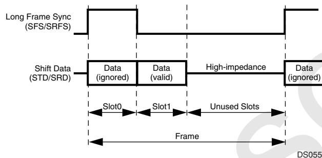
Figure 58. Network Mode Frame
