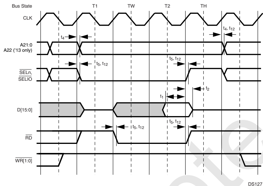
Figure 125. Normal Read Cycle (Wait Cycle Followed by Hold Cycle)
