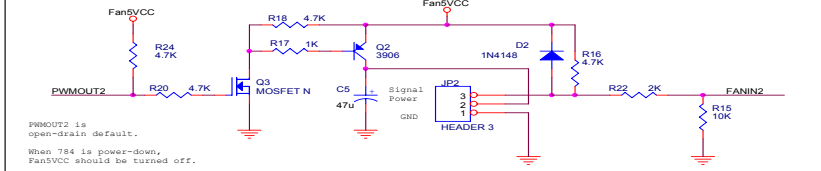
SMARTFAN2 Speed Control Circuit
