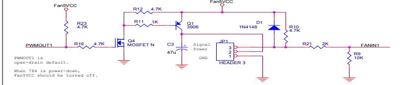
SMARTFAN1 Speed Control Circuit
