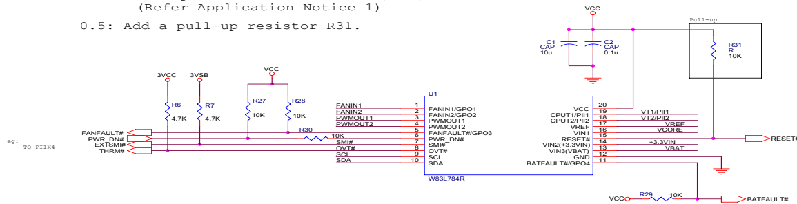
SMARTFAN1 Speed Control Circuit
