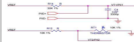
TEMPERATURE SENSING CIRCUIT
