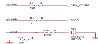
VOLTAGE SENSING CIRCUIT
