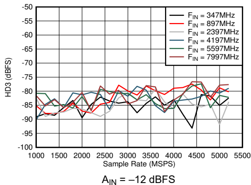
Figure 6-57. Dual Channel Mode: HD3 vs Sample Rate and Input Frequency
