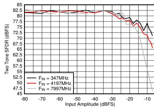
Figure 6-110. Dual Channel Mode: Two Tone SFDR vs Input Amplitude
