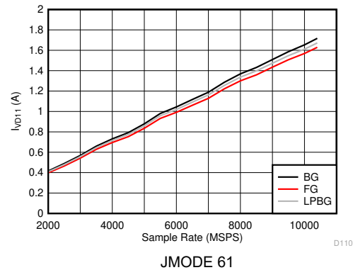
Figure 6-128. DES Mode: I_{VD11} vs Sample Rate
