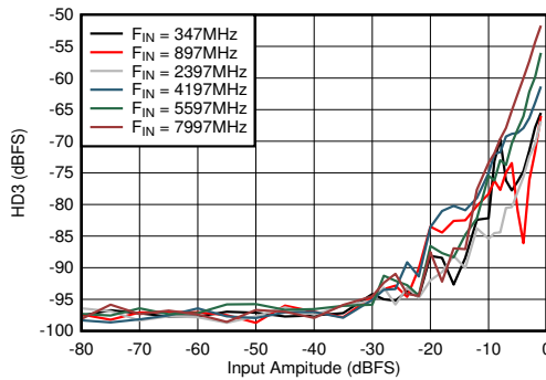
Figure 6-79. Dual Channel Mode: HD3 vs Input Amplitude and Frequency
