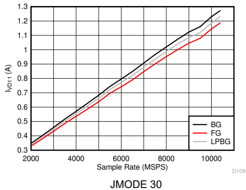
Figure 6-127. DES Mode: I_{VD11} vs Sample Rate
