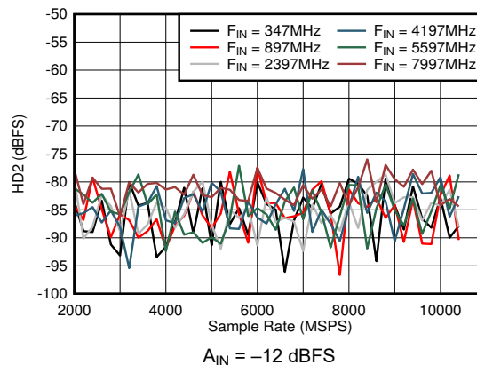
Figure 6-38. DES Mode: HD2 vs Sample Rate and Input Frequency
