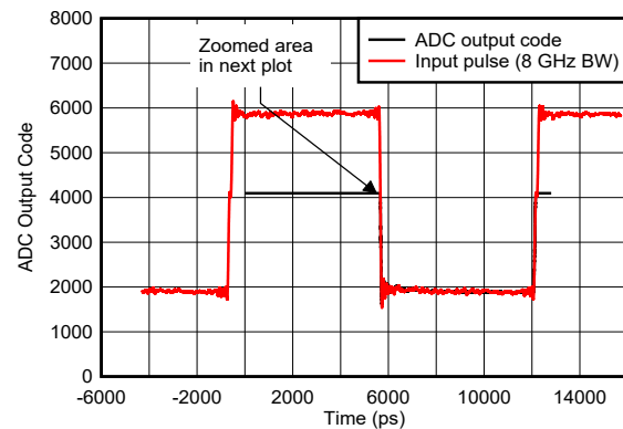
Figure 6-148. Pulse Overdrive Recovery
