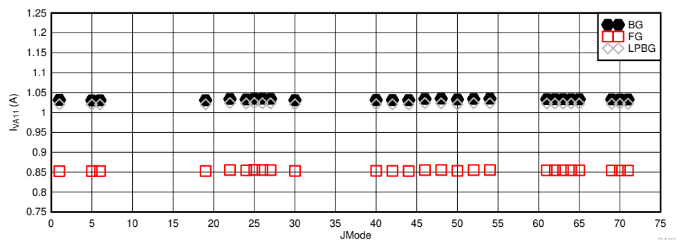
Figure 6-111. DES Mode: I_{VA19} vs JMODE at 10.4GSPS
