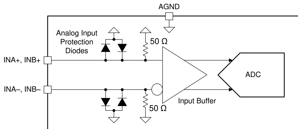
Figure 7-1. ADC12DJ5200-EP Analog Input Internal Termination and Protection Diagram
