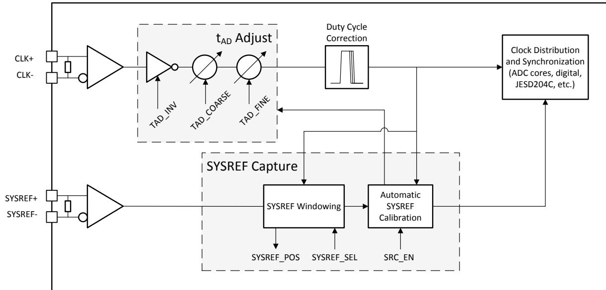
Figure 7-2. Clocking Subsystem
