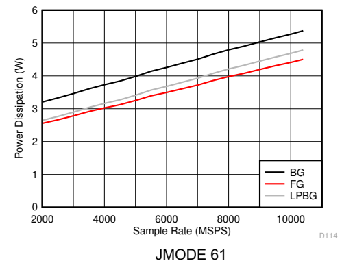
Figure 6-132. DES Mode: Power Dissipation vs Sample Rate
