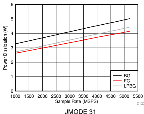
Figure 6-141. Dual Channel Mode: Power Dissipation vs Sample Rate
