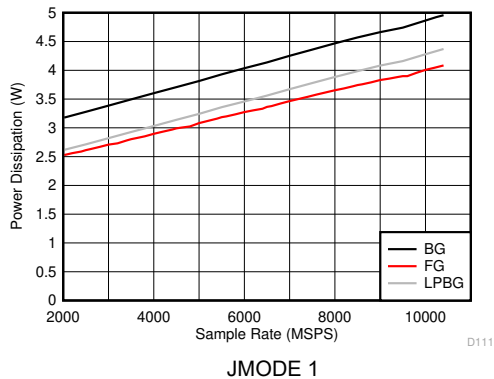
Figure 6-129. DES Mode: Power Dissipation vs Sample Rate
