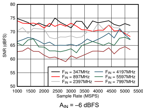
Figure 6-49. Dual Channel Mode: SNR vs Sample Rate and Input Frequency
