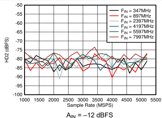
Figure 6-54. Dual Channel Mode: HD2 vs Sample Rate and Input Frequency
