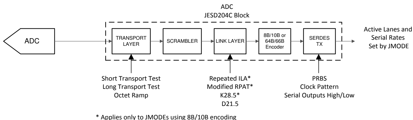
Figure 7-24. Test Mode Insertion Points
