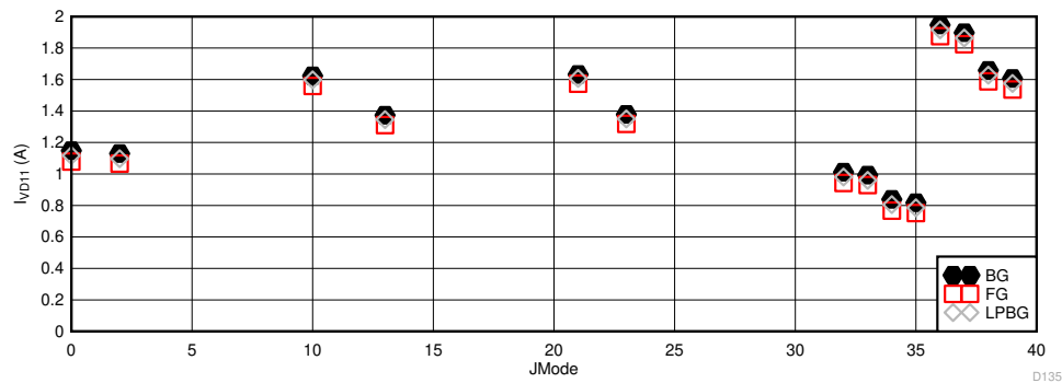
Figure 6-120. Other Modes with Lower Maximum F_S : I_{VA11} vs JMODE
