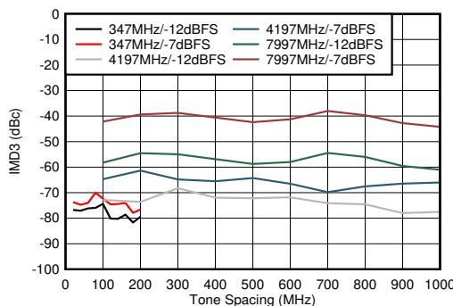
Figure 6-108. Dual Channel Mode: IMD3 vs Tone Spacing
