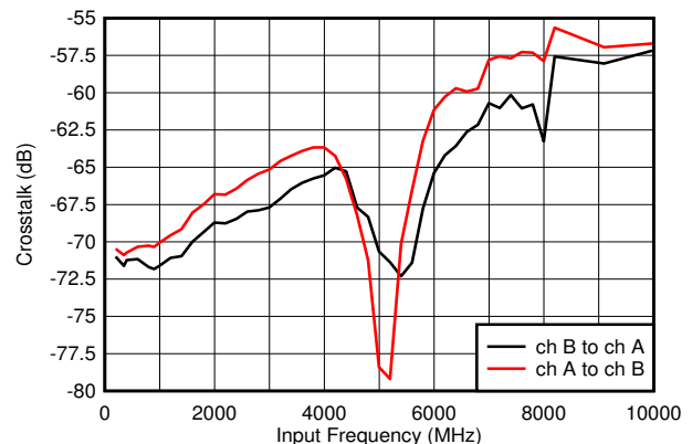
Figure 6-2. Crosstalk vs Input Frequency
