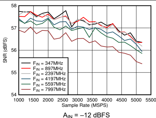
Figure 6-47. Dual Channel Mode: SNR vs Sample Rate and Input Frequency
