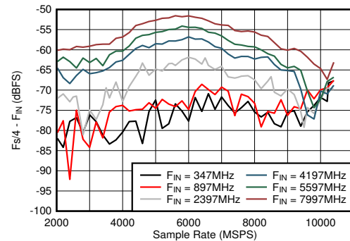
Figure 6-44. DES Mode: F_s/4 - F_{\text{IN}} vs Sample Rate and Input Frequency
