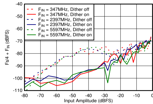
Figure 6-68. DES Mode: F_s/2 - F_{\text{IN}} vs Input Amplitude and Dither
