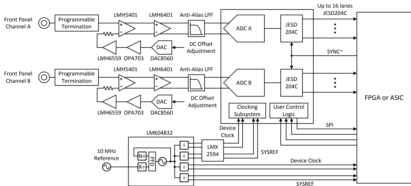
Figure 8-2. Typical Configuration for Reconfigurable Oscilloscope
