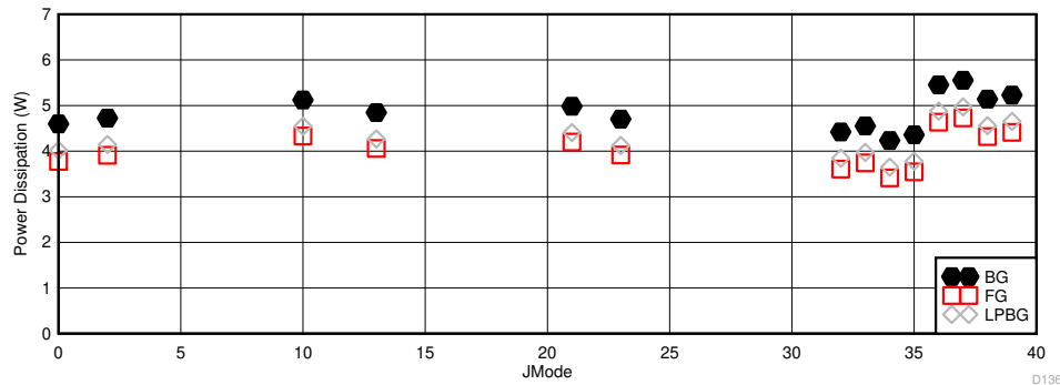
Figure 6-122. Other Modes with Lower Maximum F_S : Power Dissipation vs JMODE
