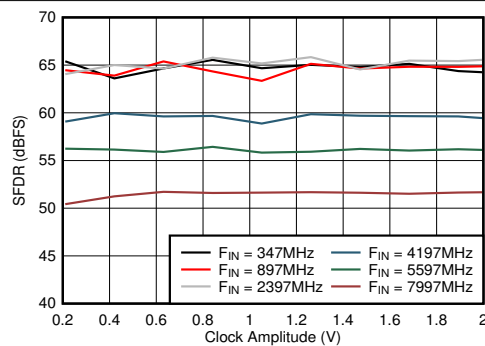
Figure 6-86. Dual Channel Mode: SFDR vs Clock Amplitude
