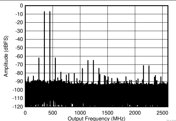
Figure 6-25. Dual Channel Mode: Two Tone FFT at 2397 MHz
