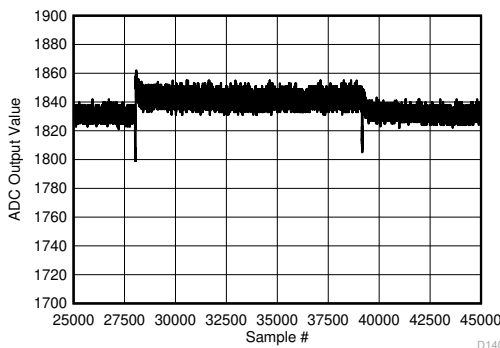
Figure 6-147. Background Calibration Core Transition (DC Signal - zoomed)
