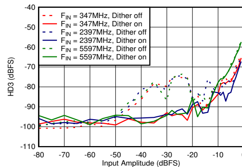
Figure 6-66. DES Mode: HD3 vs Input Amplitude and Dither
