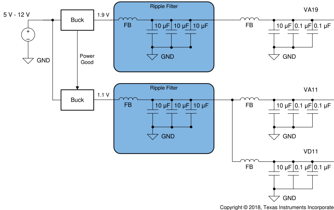
Figure 8-4. Switcher-Only Approach Example
