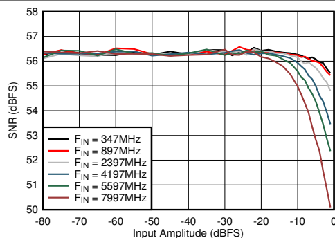
Figure 6-59. DES Mode: SNR vs Input Amplitude and Frequency
