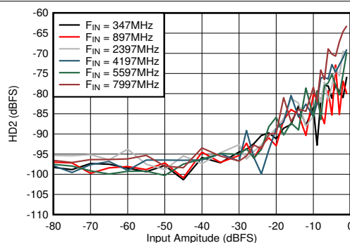
Figure 6-63. DES Mode: HD2 vs Input Amplitude and Frequency
