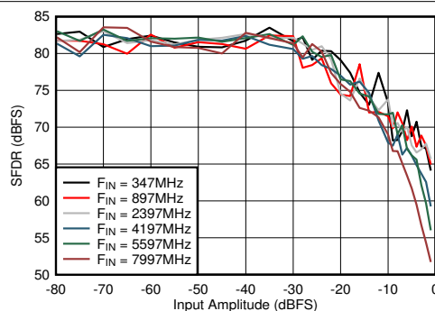
Figure 6-75. Dual Channel Mode: SFDR vs Input Amplitude and Frequency
