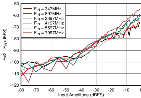
Figure 6-67. DES Mode: F_s/2 - F_{\text{IN}} vs Input Amplitude and Frequency
