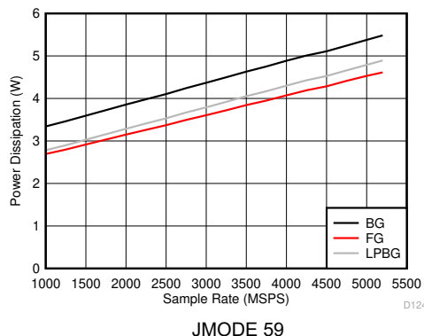
Figure 6-142. Dual Channel Mode: Power Dissipation vs Sample Rate
