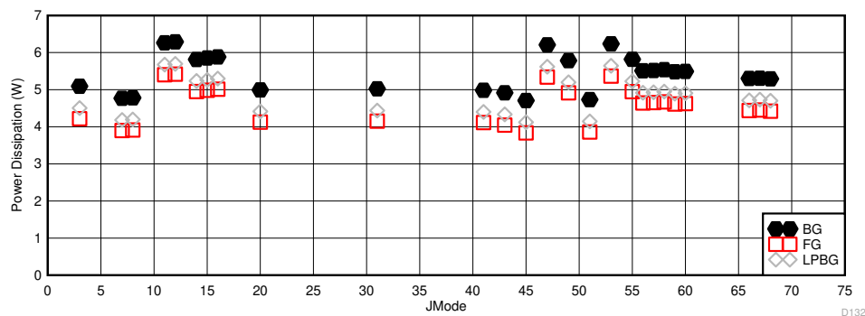
Figure 6-117. Dual Channel Mode: I_{VD11} vs JMODE at 5.2GSPS
