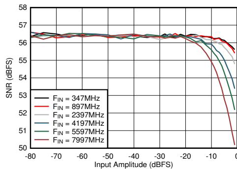
Figure 6-73. Dual Channel Mode: SNR vs Input Amplitude and Frequency
