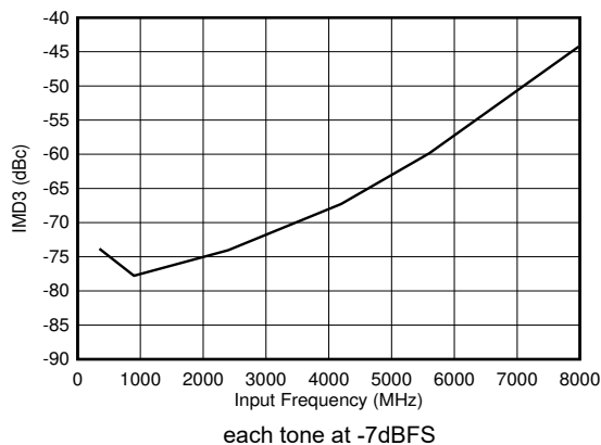
Figure 6-101. DES Mode: IMD3 vs Input Frequency
