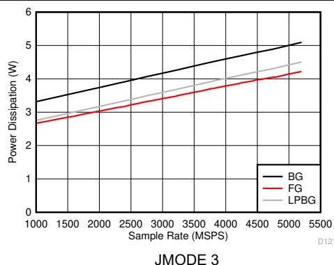
Figure 6-139. Dual Channel Mode: Power Dissipation vs Sample Rate
