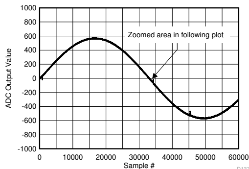
Figure 6-144. Background Calibration Core Transition (AC Signal)
