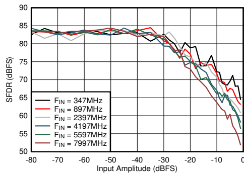
Figure 6-61. DES Mode: SFDR vs Input Amplitude and Frequency
