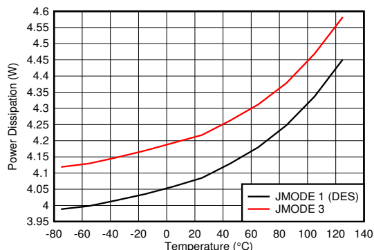
Figure 6-143. Power Dissipation vs Temperature
