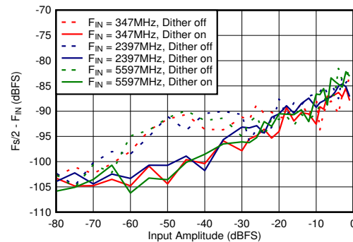
Figure 6-82. Dual Channel Mode: F_s/2 - F_{\text{IN}} vs Input Amplitude and Dither
