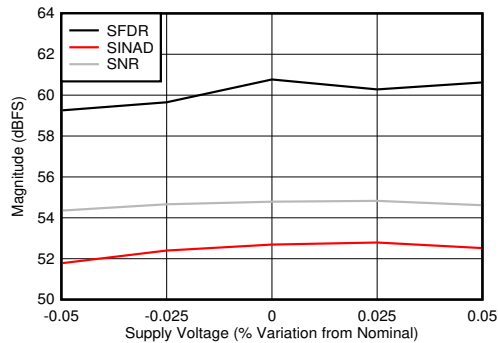
Figure 6-95. DES Mode: SNR, SINAD and SFDR vs Supply Voltage
