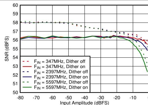
Figure 6-60. DES Mode: SNR vs Input Amplitude and Dither
