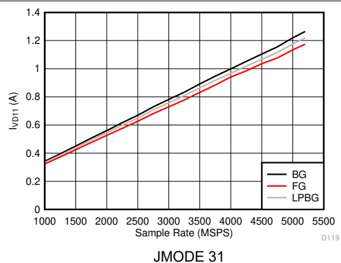
Figure 6-137. Dual Channel Mode: I_{VD11} vs Sample Rate
