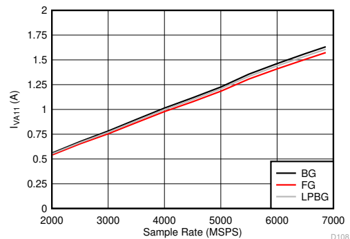
Figure 6-124. DES Mode: I_{VA11} vs Sample Rate
