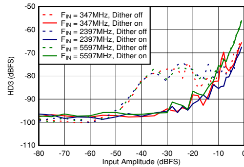
Figure 6-80. Dual Channel Mode: HD3 vs Input Amplitude and Dither
