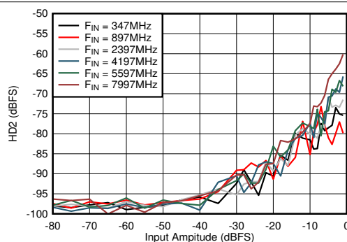
Figure 6-77. Dual Channel Mode: HD2 vs Input Amplitude and Frequency
