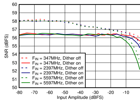
Figure 6-74. Dual Channel Mode: SNR vs Input Amplitude and Dither
