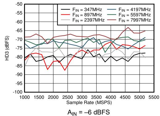
Figure 6-56. Dual Channel Mode: HD3 vs Sample Rate and Input Frequency
