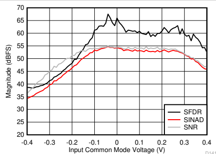
Figure 6-99. SNR, SFDR and SINAD vs Input Common Mode Voltage
