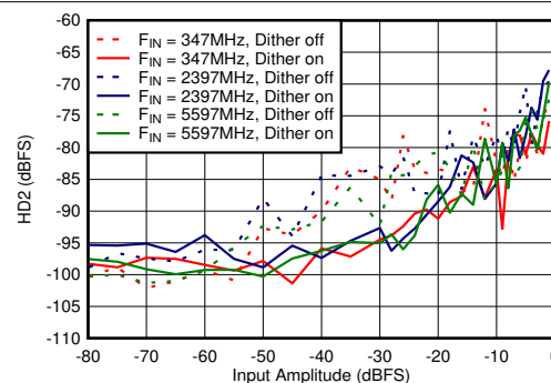
Figure 6-64. DES Mode: HD2 vs Input Amplitude and Dither
