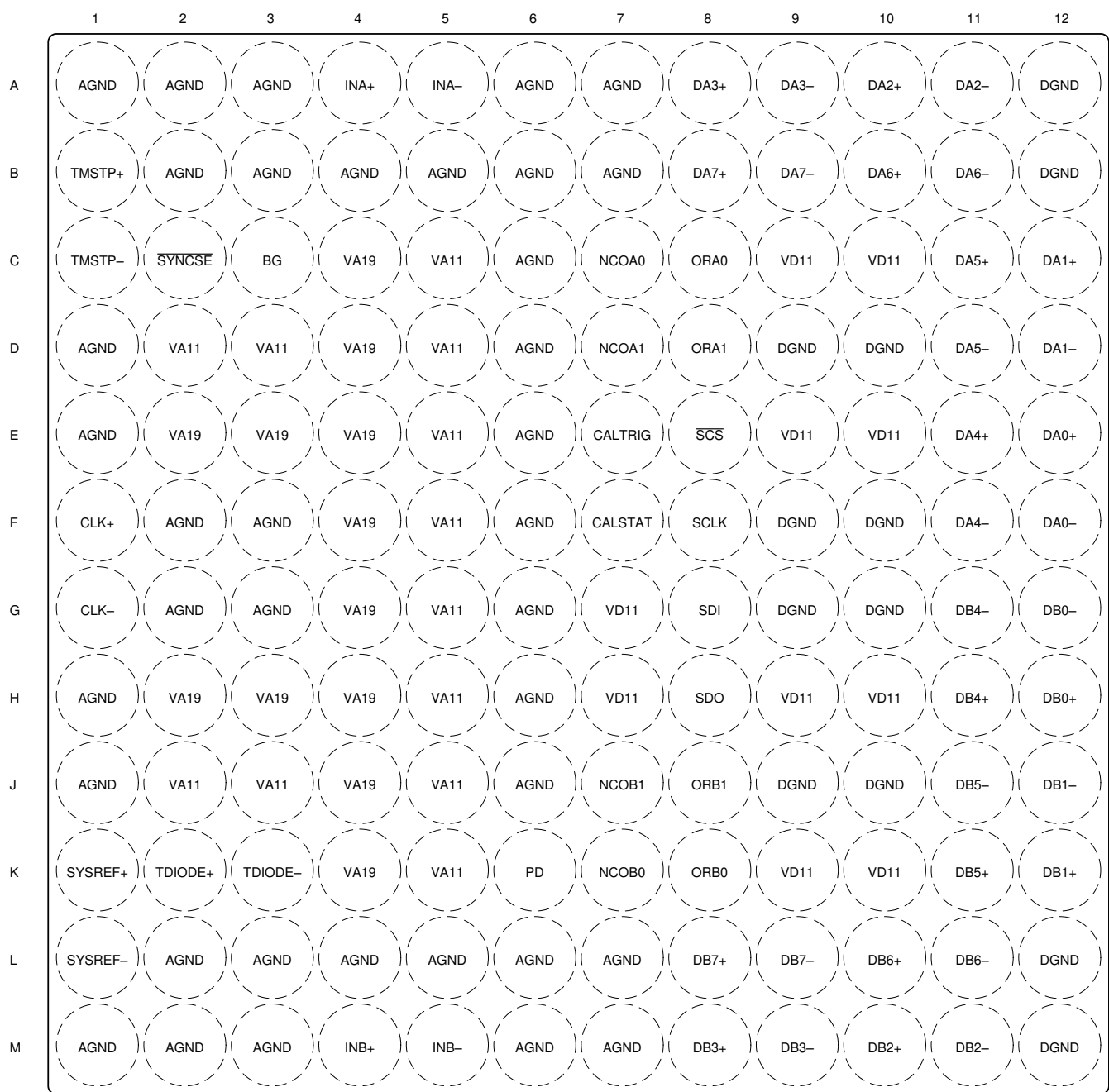
Figure 5-1. ALR Package, 144-Ball Flip Chip BGA Top View
