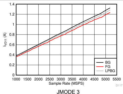
Figure 6-135. Dual Channel Mode: I_{VD11} vs Sample Rate
