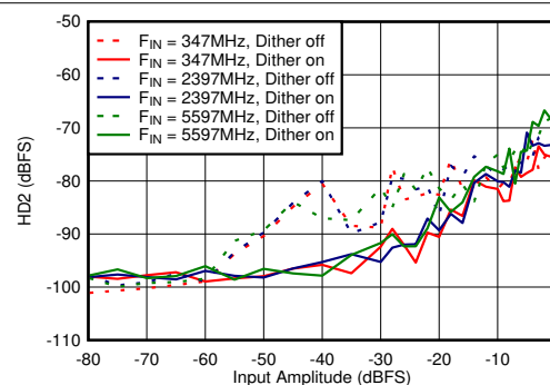
Figure 6-78. Dual Channel Mode: HD2 vs Input Amplitude and Dither
