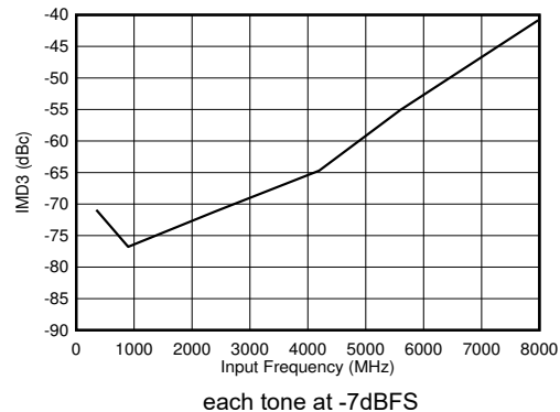
Figure 6-106. Dual Channel Mode: IMD3 vs Input Frequency
