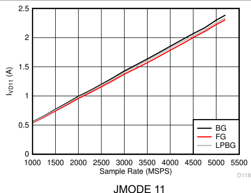
Figure 6-136. Dual Channel Mode: I_{VD11} vs Sample Rate
