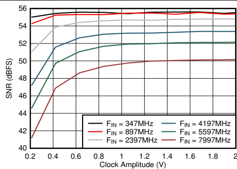
Figure 6-85. Dual Channel Mode: SNR vs Clock Amplitude
