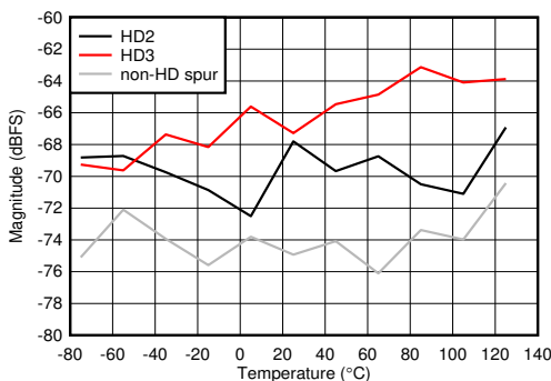
Figure 6-89. DES Mode: HD2, HD3 and Worst non-HD Spur vs Temperature
