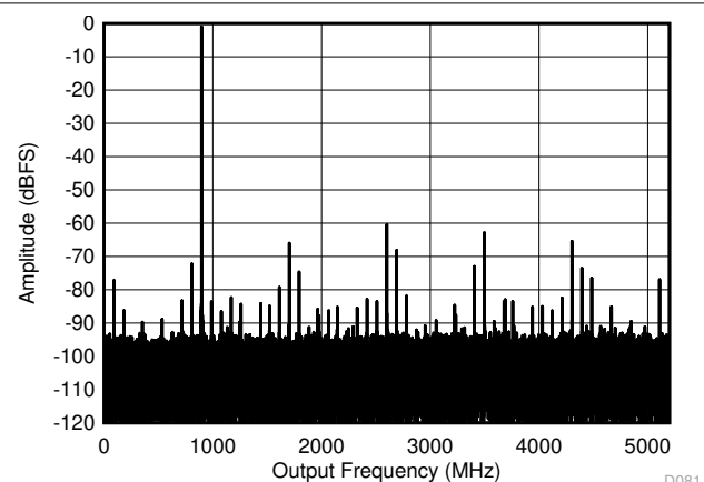
Figure 6-6. DES Mode: Single Tone FFT at 897 MHz
