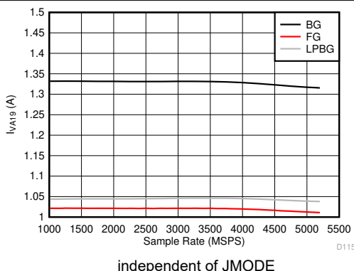
Figure 6-133. Dual Channel Mode: I_{VA19} vs Sample Rate
