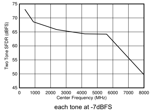
Figure 6-104. DES Mode: Two Tone SFDR vs Input Frequency
