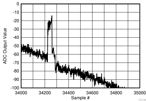
Figure 6-145. Background Calibration Core Transition (AC Signal - zoomed)
