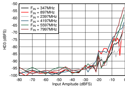
Figure 6-65. DES Mode: HD3 vs Input Amplitude and Frequency
