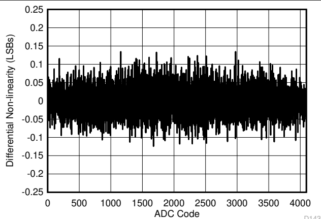
Figure 6-3. DNL vs ADC Code
