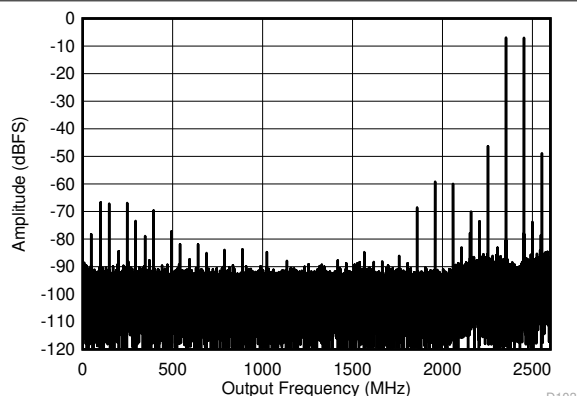
Figure 6-26. Dual Channel Mode: Two Tone FFT at 4197 MHz
