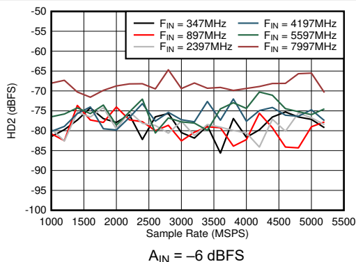
Figure 6-53. Dual Channel Mode: HD2 vs Sample Rate and Input Frequency
