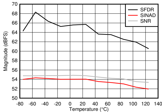
Figure 6-91. Dual Channel Mode: SNR, SINAD and SFDR vs Temperature
