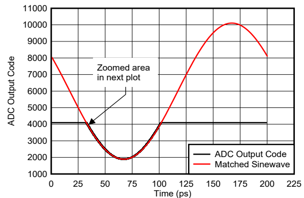
Figure 6-150. Sinewave Overdrive Recovery
