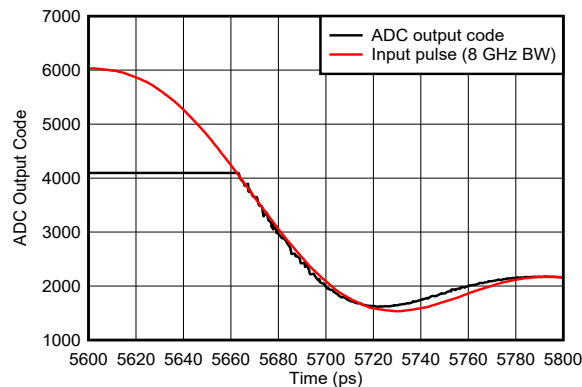
Figure 6-149. Pulse Overdrive Recovery Zoomed
