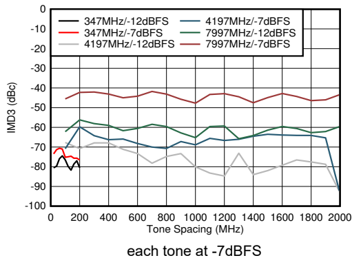
Figure 6-103. DES Mode: IMD3 vs Tone Spacing
