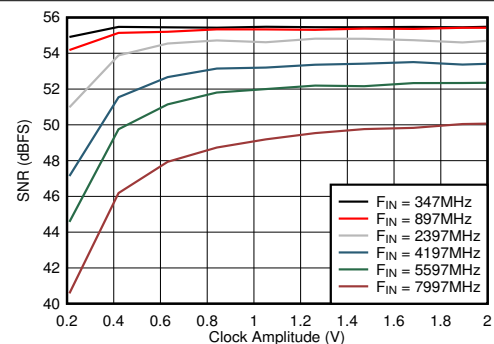
Figure 6-83. DES Mode: SNR vs Clock Amplitude
