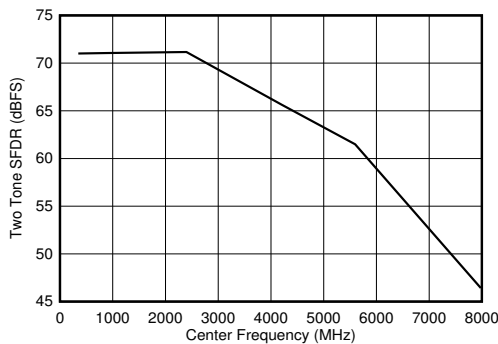
Figure 6-109. Dual Channel Mode: Two Tone SFDR vs Input Frequency
