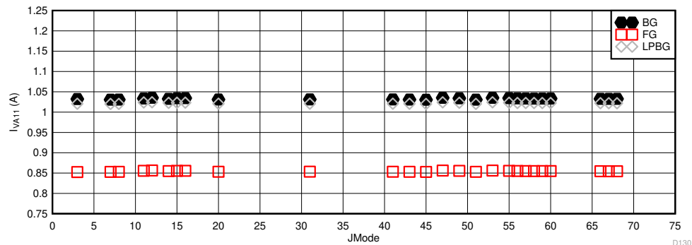
Figure 6-116. Dual Channel Mode: I_{VA11} vs JMODE at 5.2GSPS
