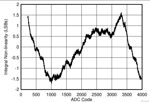
Figure 6-4. INL vs ADC Code
