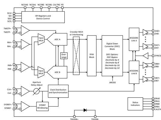
ADC12DJ5200-EP Block Diagram
