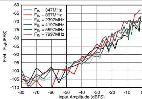
Figure 6-71. DES Mode: F_s/4 - F_{\text{IN}} vs Input Amplitude and Frequency
