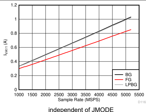
Figure 6-134. Dual Channel Mode: I_{VA11} vs Sample Rate
