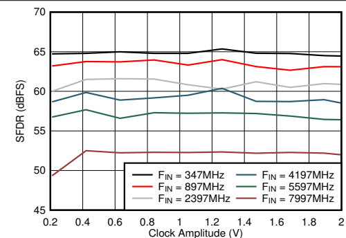
Figure 6-84. DES Mode: SFDR vs Clock Amplitude
