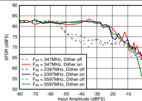
Figure 6-76. Dual Channel Mode: SFDR vs Input Amplitude and Dither
