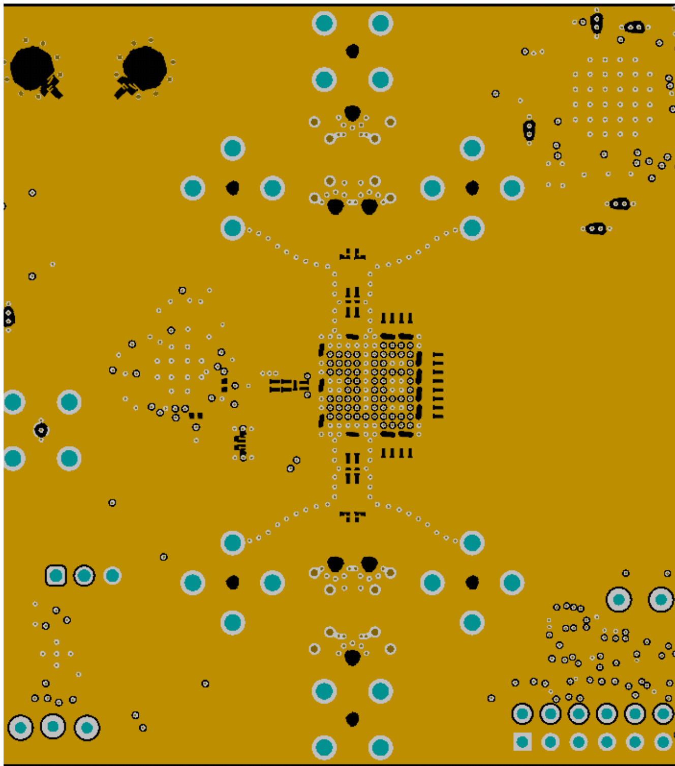
Figure 8-6. GND1 Cutouts to Optimize Impedance of Component Pads
