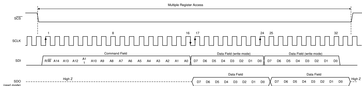
Figure 7-27. Serial Interface Protocol: Streaming Read/Write
