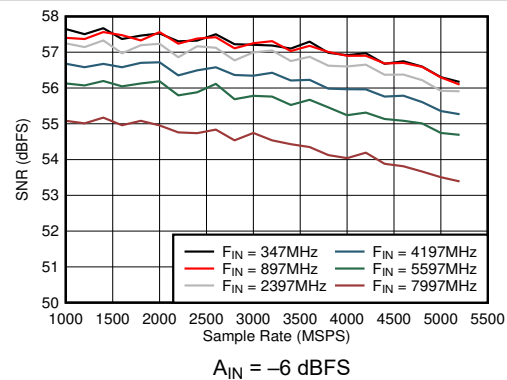
Figure 6-46. Dual Channel Mode: SNR vs Sample Rate and Input Frequency
