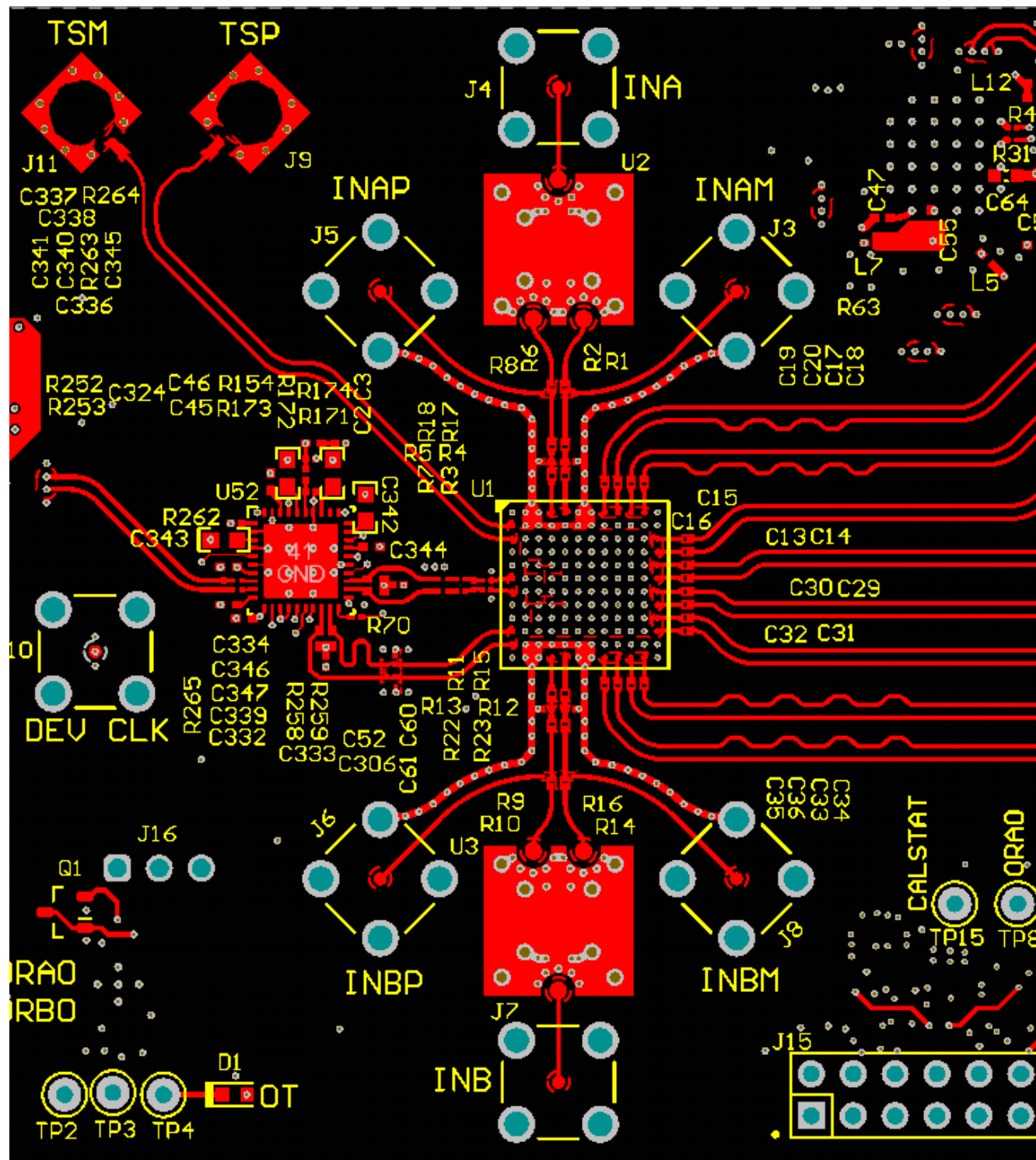
Figure 8-5. Top Layer Routing: Analog Inputs, CLK and SYSREF, DA0-3, DB0-3
