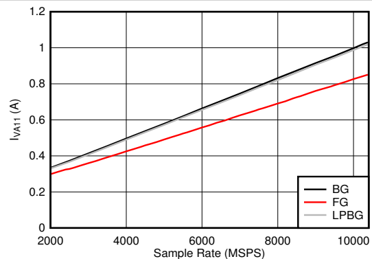
Figure 6-124. DES Mode: I_{VA11} vs Sample Rate
