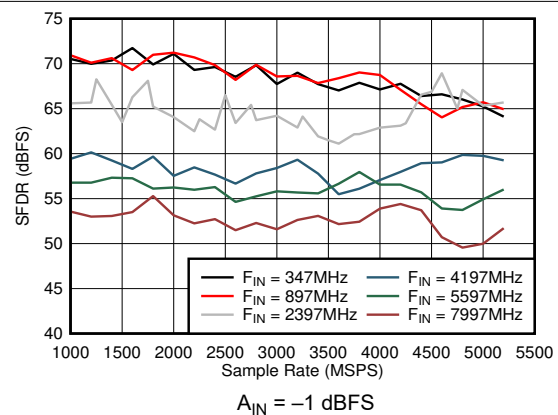
Figure 6-48. Dual Channel Mode: SFDR vs Sample Rate and Input Frequency
