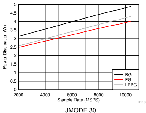
Figure 6-131. DES Mode: Power Dissipation vs Sample Rate
