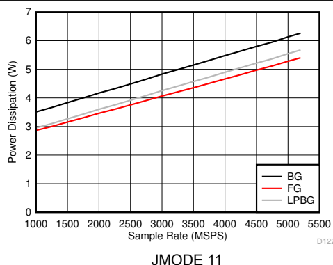
Figure 6-140. Dual Channel Mode: Power Dissipation vs Sample Rate
