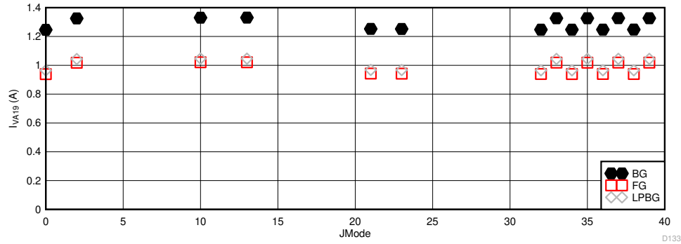
Figure 6-119. Other Modes with Lower Maximum F_S : I_{VA19} vs JMODE
