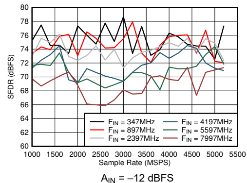
Figure 6-50. Dual Channel Mode: SFDR vs Sample Rate and Input Frequency
