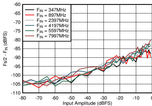
Figure 6-81. Dual Channel Mode: F_s/2 - F_{\text{IN}} vs Input Amplitude and Frequency
