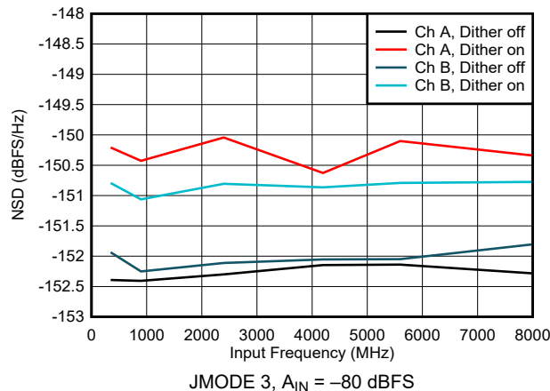
Figure 6-51. Dual Channel Mode: NSD and Input Frequency
