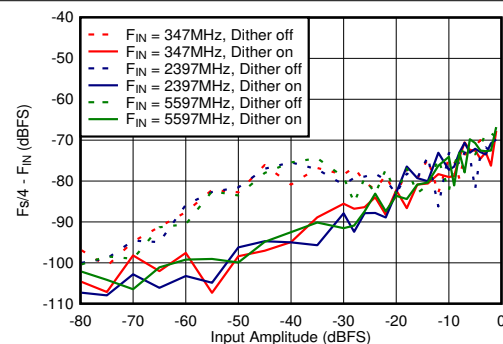
Figure 6-72. DES Mode: F_s/4 - F_{\text{IN}} vs Input Amplitude and Dither
