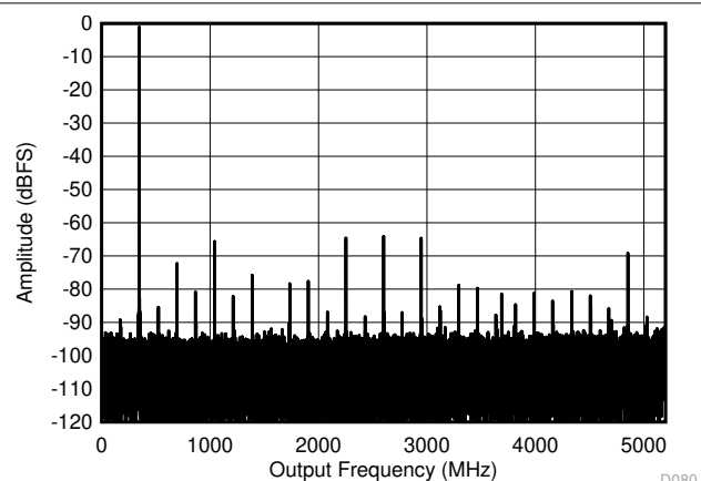
Figure 6-5. DES Mode: Single Tone FFT at 347 MHz
