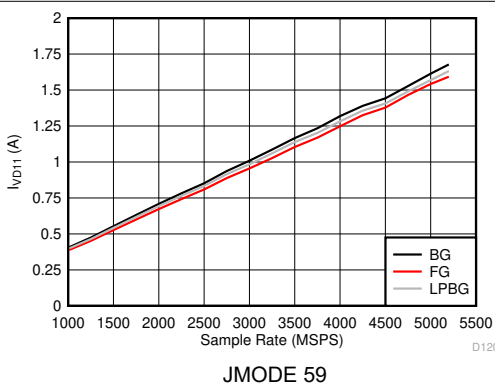
Figure 6-138. Dual Channel Mode: I_{VD11} vs Sample Rate
