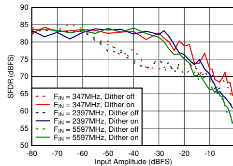
Figure 6-62. DES Mode: SFDR vs Input Amplitude and Dither
