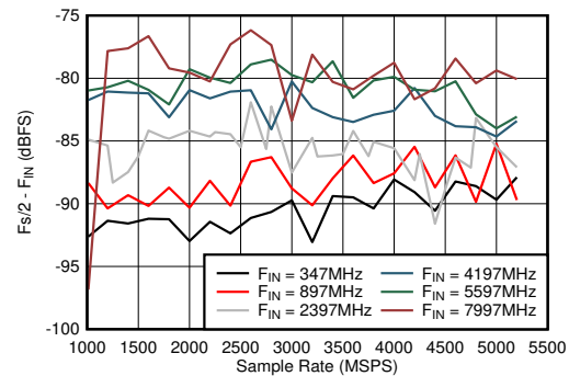
Figure 6-58. Dual Channel Mode: F_s/2 - F_{\text{IN}} vs Sample Rate and Input Frequency
