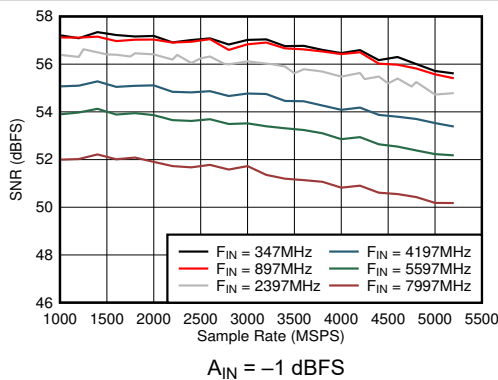
Figure 6-45. Dual Channel Mode: SNR vs Sample Rate and Input Frequency
