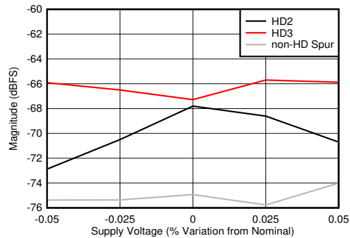
Figure 6-96. DES Mode: HD2, HD3 and Worst non-HD Spur vs Supply Voltage
