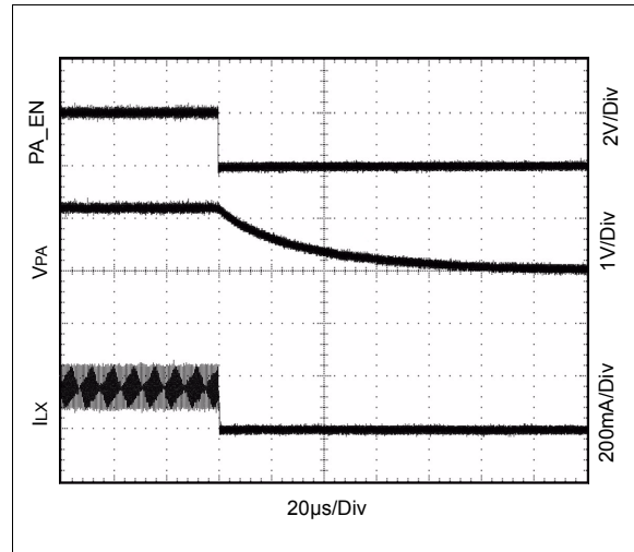
Figure 34. DC-DC Shutdown
