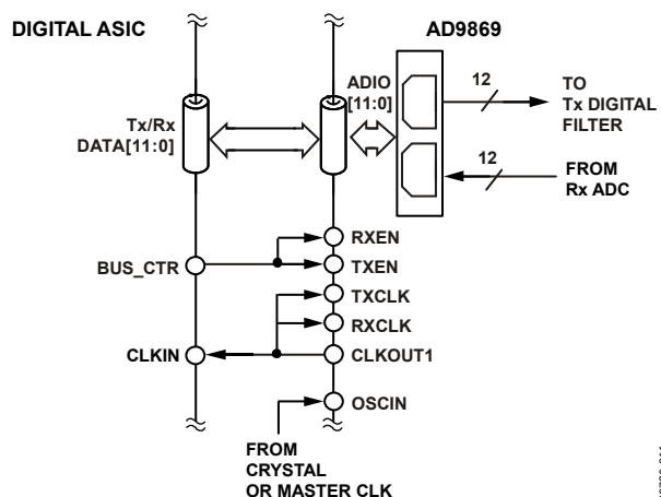
Figure 11. Example of a Half-Duplex Digital Interface with AD9869 Serving as the Master
