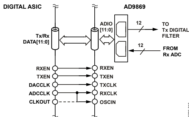
Figure 10. Example of a Half-Duplex Digital Interface with AD9869 Serving as the Slave
