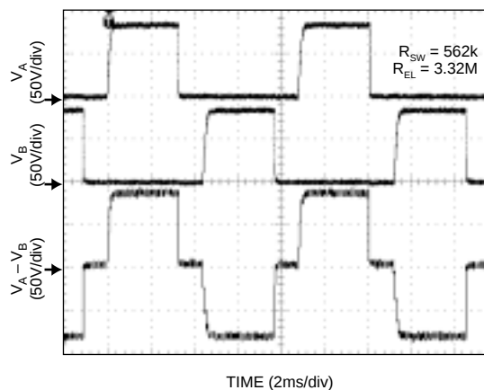
Figure 2. Typical MIC4826 Output Waveform for V_{IN} = 5.5V
