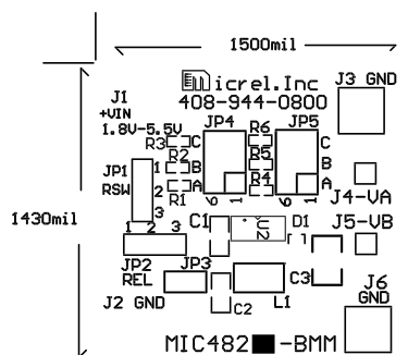
Top Side Silk Screen
