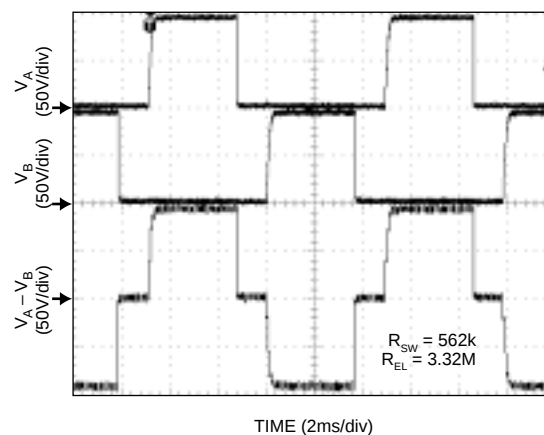
Figure 4. Typical MIC4827 Output Waveform for V_{IN} = 5.5V
