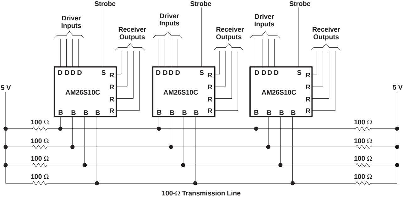
Figure 2. Party-Line System
