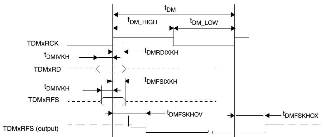
Figure 37. TDM Receive Signals
