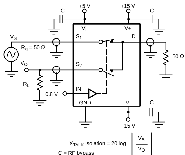
FIGURE 7. Crosstalk
