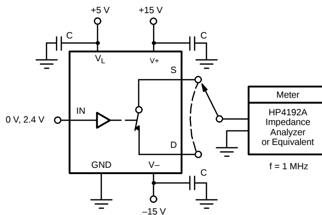
FIGURE 8. Capacitances
