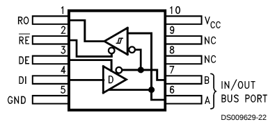
10-Lead Ceramic Flatpak
