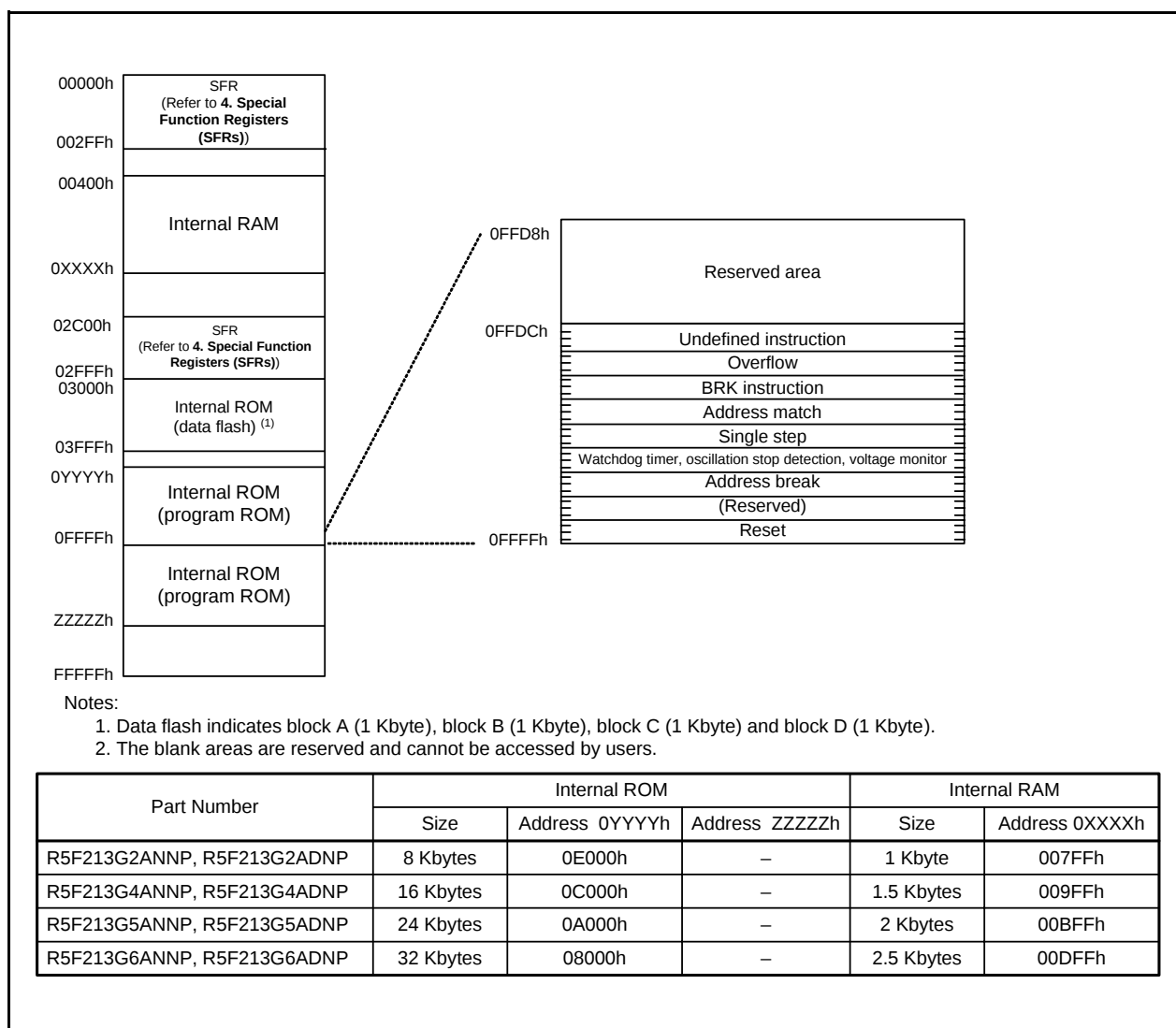
Figure 3.1 Memory Map of R8C/3GA Group
