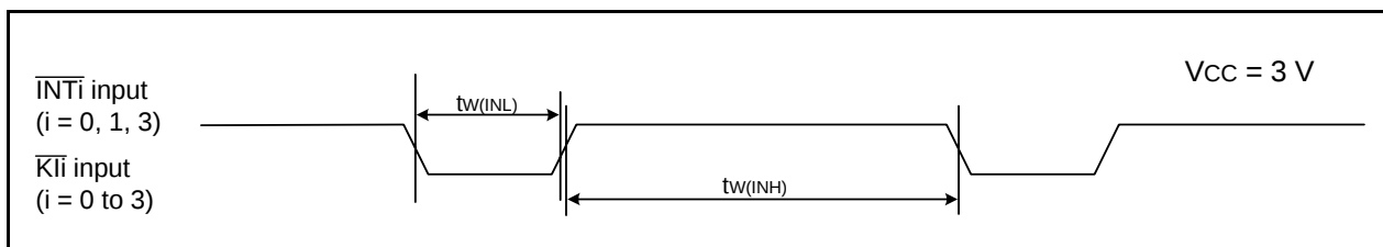
Figure 5.15 Input Timing for External Interrupt \overline{INTi} and Key Input Interrupt \overline{Kli} when V_{CC} = 3\text{ V}
