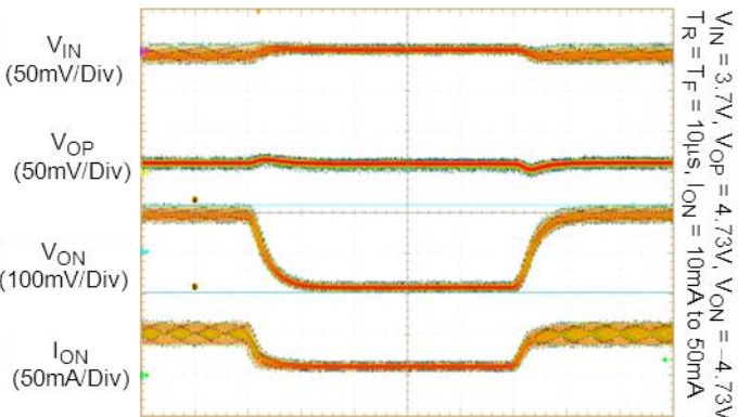
V ON Load Transient
