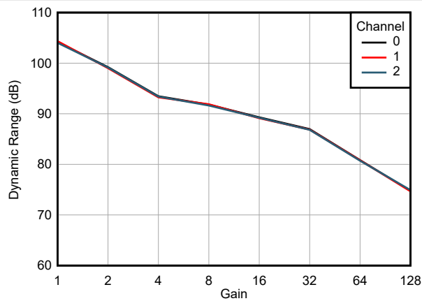
Figure 6-22. Dynamic Range vs Gain
