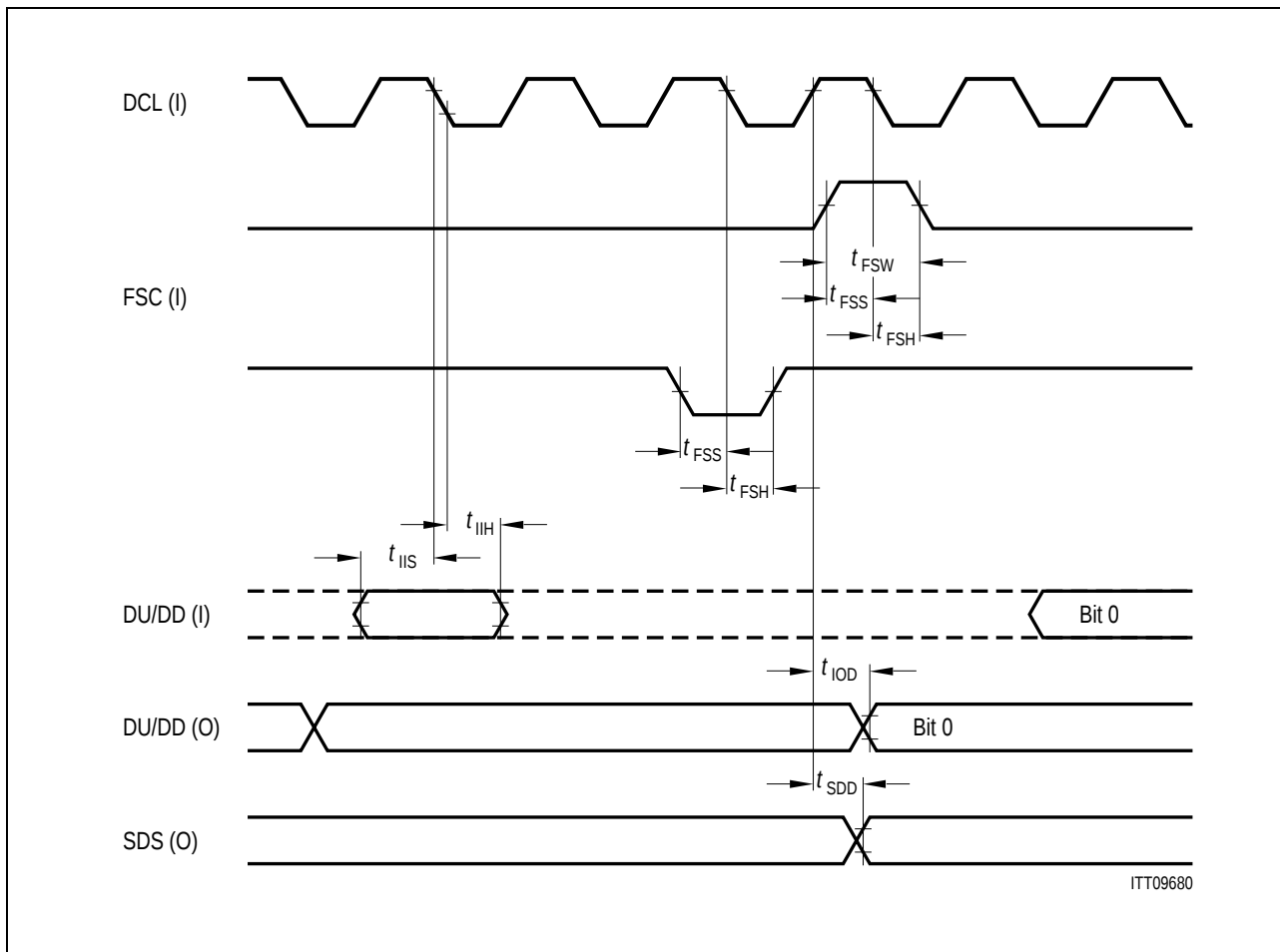
Figure 71 IOM-2 Timing (LT-S, LT-T, NT mode)
