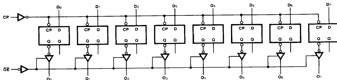
LOGIC DIAGRAM
