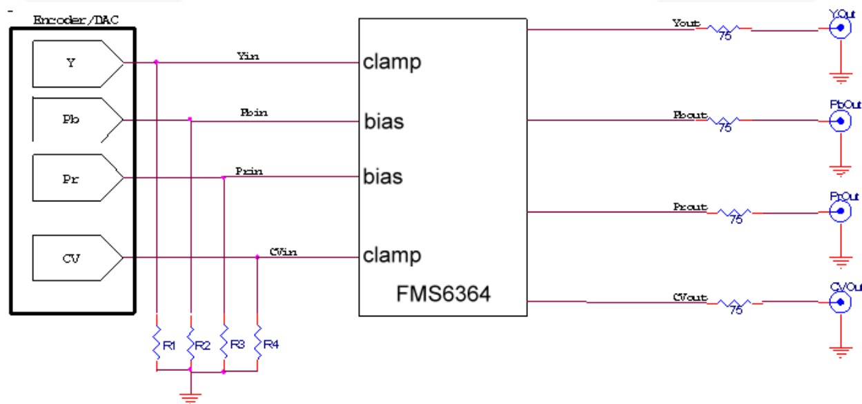
Figure 11. Typical Application
