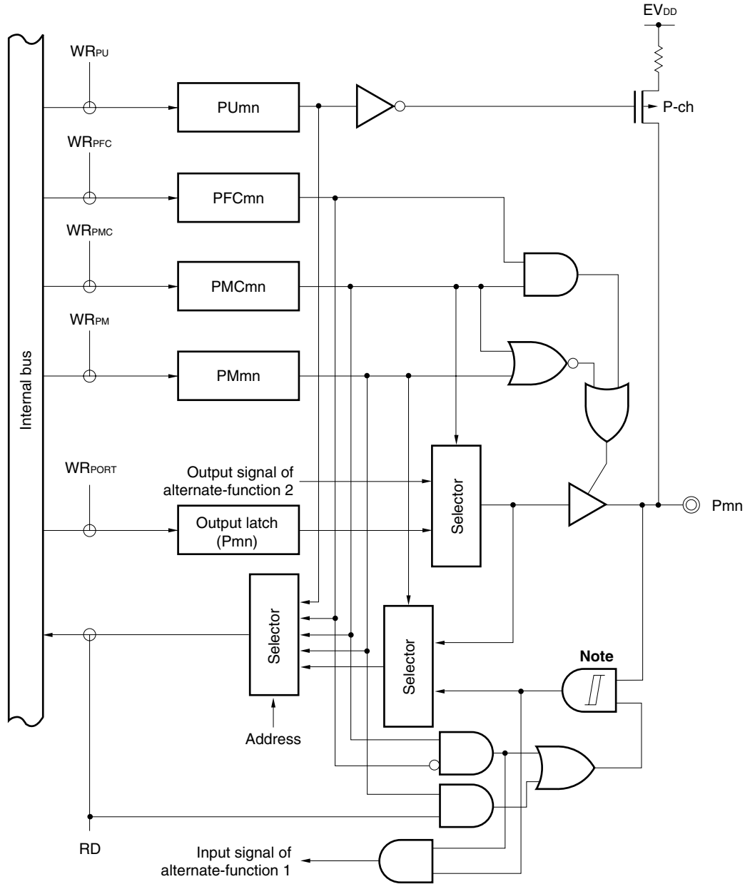
Figure 4-17. Block Diagram of Type E-6
