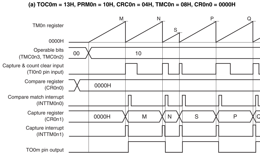
Figure 8-16. Timing Example of Clear & Start Mode Entered by TI0n0 Pin Valid Edge Input (CR0n0 Register: Compare Register, CR0n1 Register: Capture Register) (1/2)
