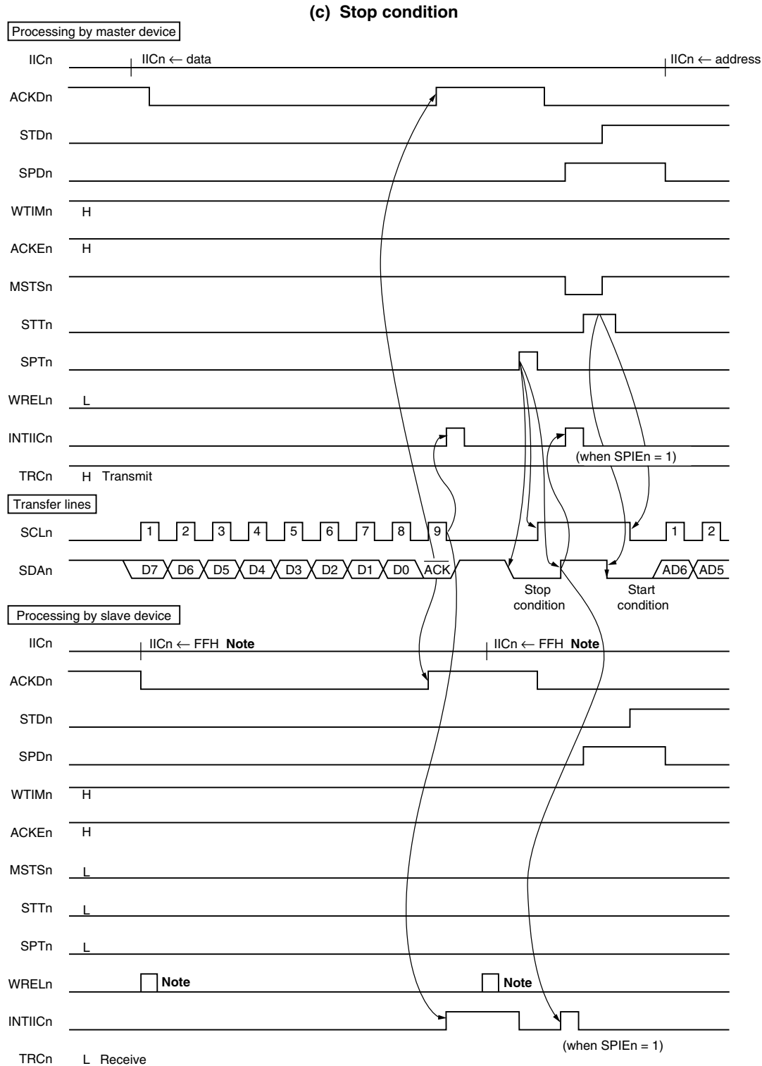
Figure 19-21. Example of Master to Slave Communication (When 9-Clock Wait Is Selected for Both Master and Slave) (3/3)
