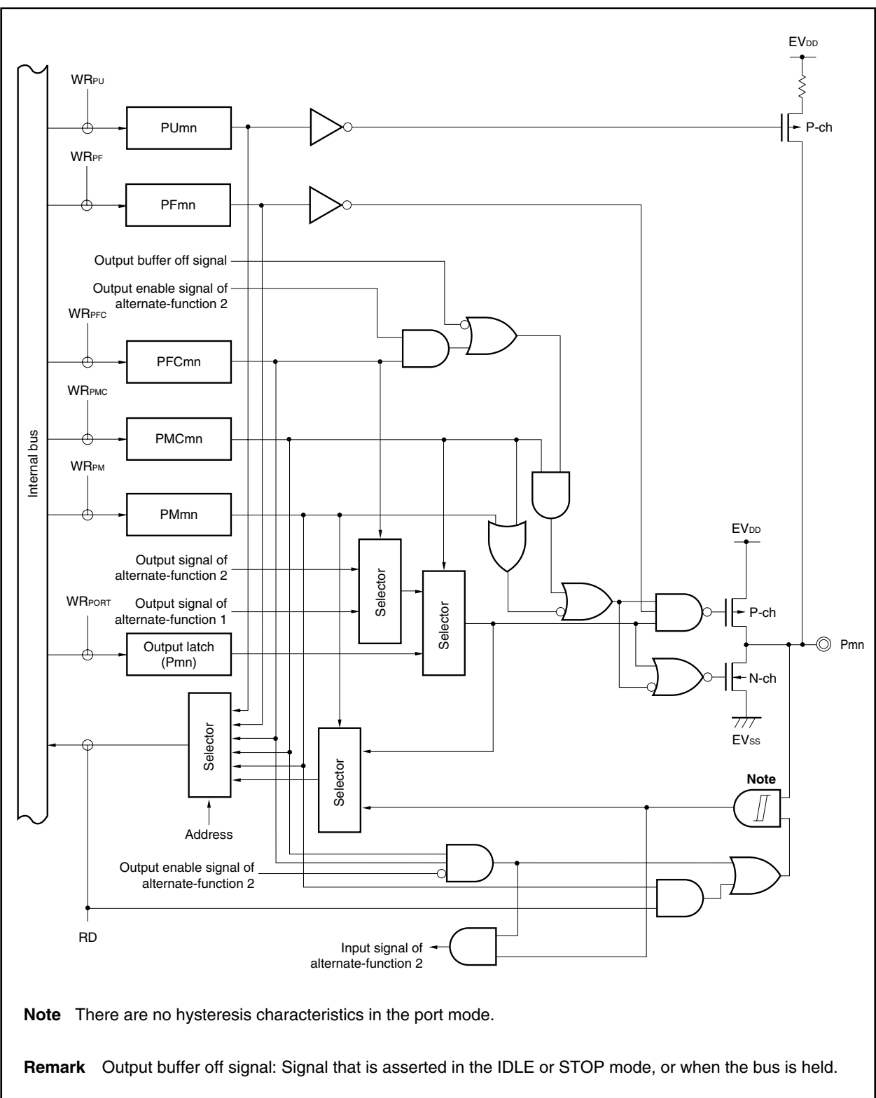
Figure 4-22. Block Diagram of Type G-3
