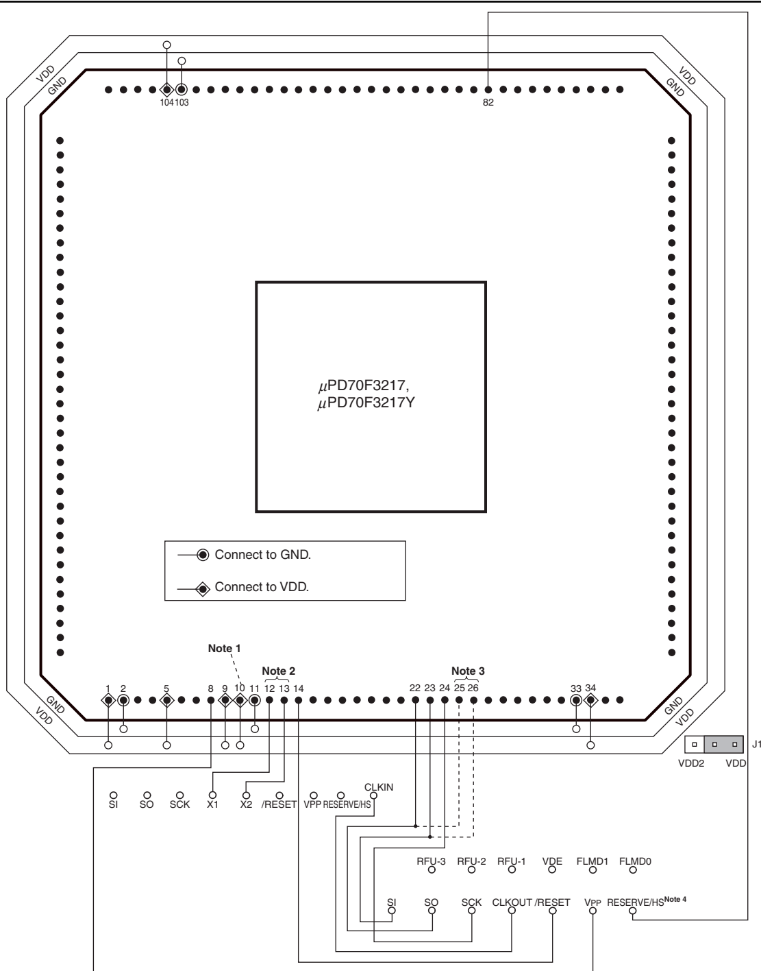
Figure 27-1. Wiring Example of V850ES/KJ1 Flash Writing Adapter (FA-144GJ-UEN-A) (1/2)
