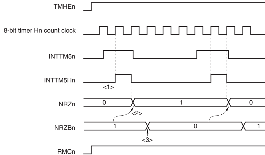
Figure 10-6. Transfer Timing
