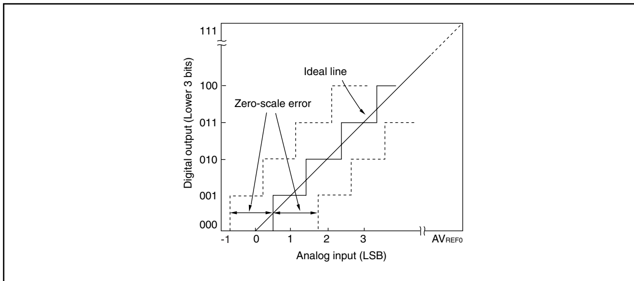
Figure 14-12. Zero-Scale Error
