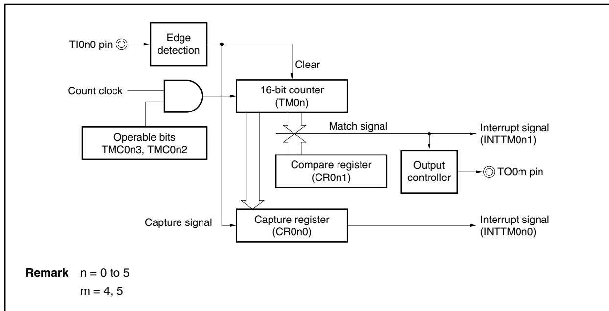
Figure 8-17. Block Diagram of Clear & Start Mode Entered by TI0n0 Pin Valid Edge Input (CR0n0 Register: Capture Register, CR0n1 Register: Compare Register)
