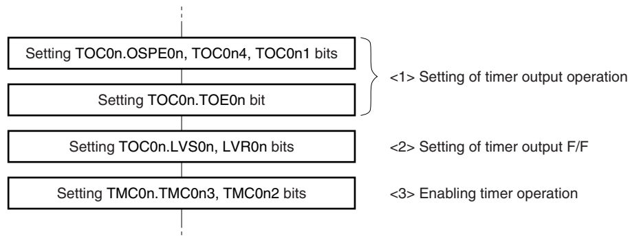
Figure 8-44. Example of Flow for Setting LVS0n and LVR0n Bits
