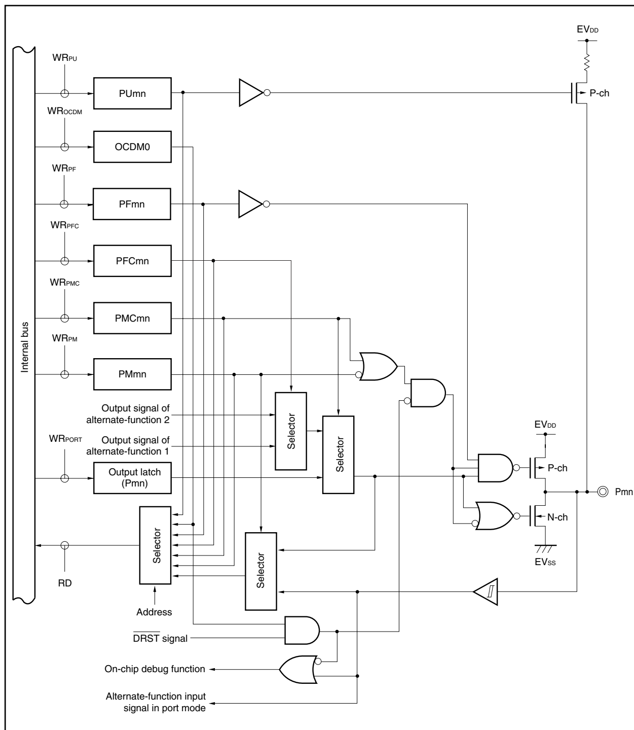
Figure 4-33. Block Diagram of Type O-2
