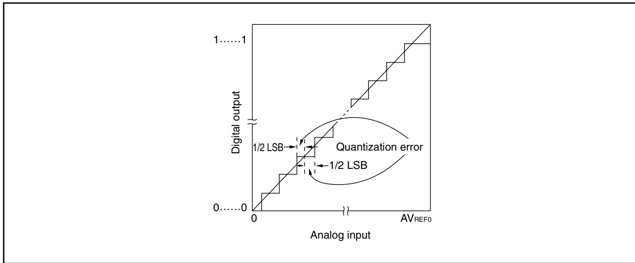
Figure 14-11. Quantization Error
