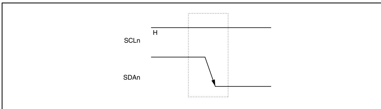
Figure 19-6. Start Conditions
