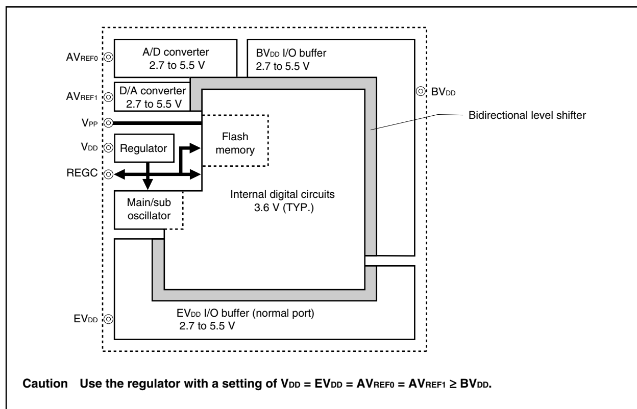
Figure 24-1. Regulator
