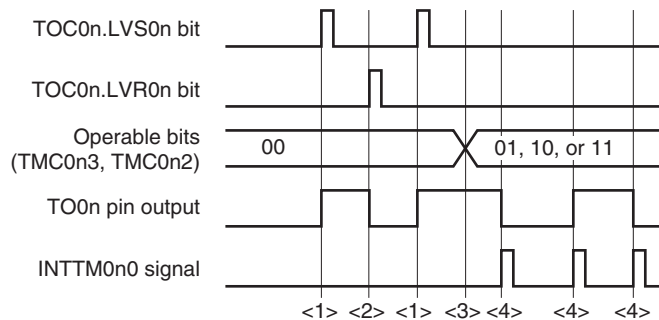
Figure 8-45. Timing Example of LVR0n and LVS0n Bits
