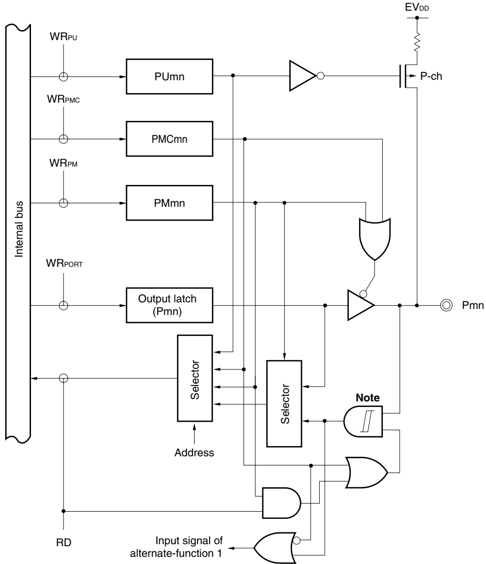
Figure 4-9. Block Diagram of Type D-1-1
