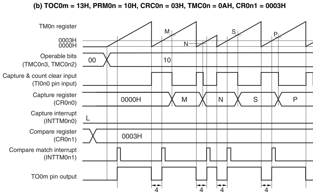
Figure 8-18. Timing Example of Clear & Start Mode Entered by TI0n0 Pin Valid Edge Input (CR0n0 Register: Capture Register, CR0n1 Register: Compare Register) (2/2)
