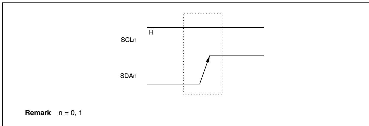
Figure 19-10. Stop Condition
