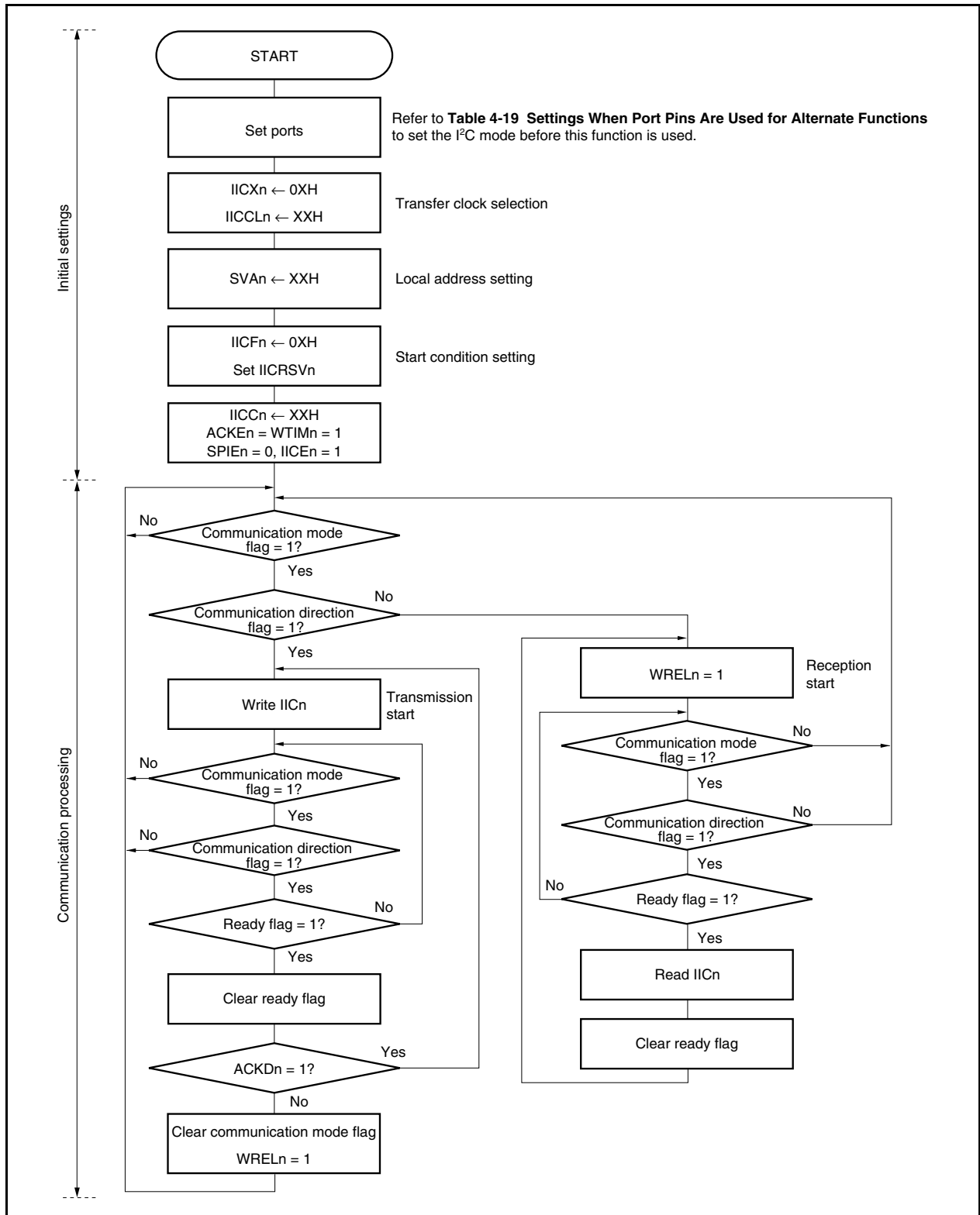
Figure 19-19. Slave Operation Flowchart (1)
