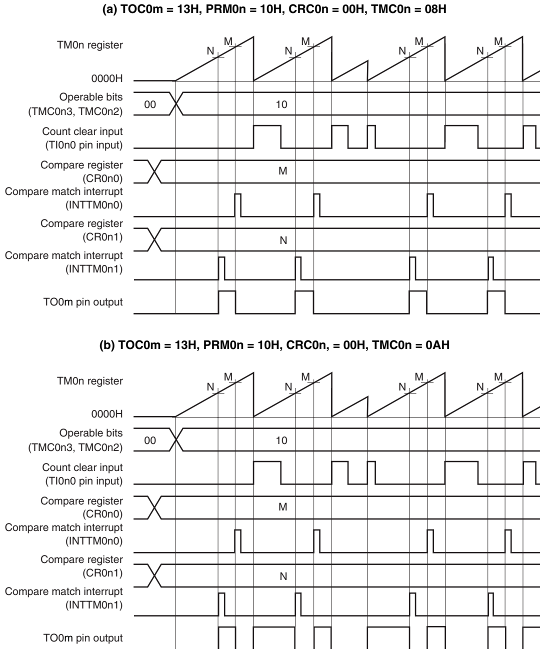
Figure 8-14. Timing Example of Clear & Start Mode Entered by TI0n0 Pin Valid Edge Input (CR0n0 Register: Compare Register, CR0n1 Register: Compare Register)
