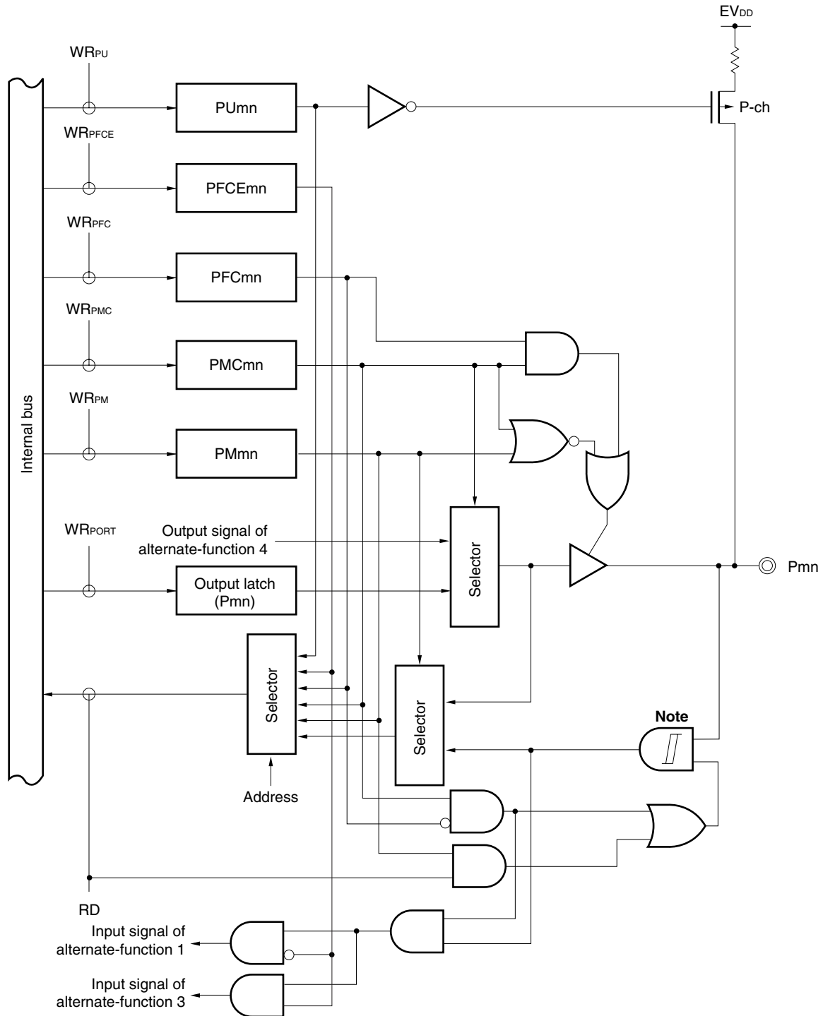
Figure 4-27. Block Diagram of Type G-7-2
