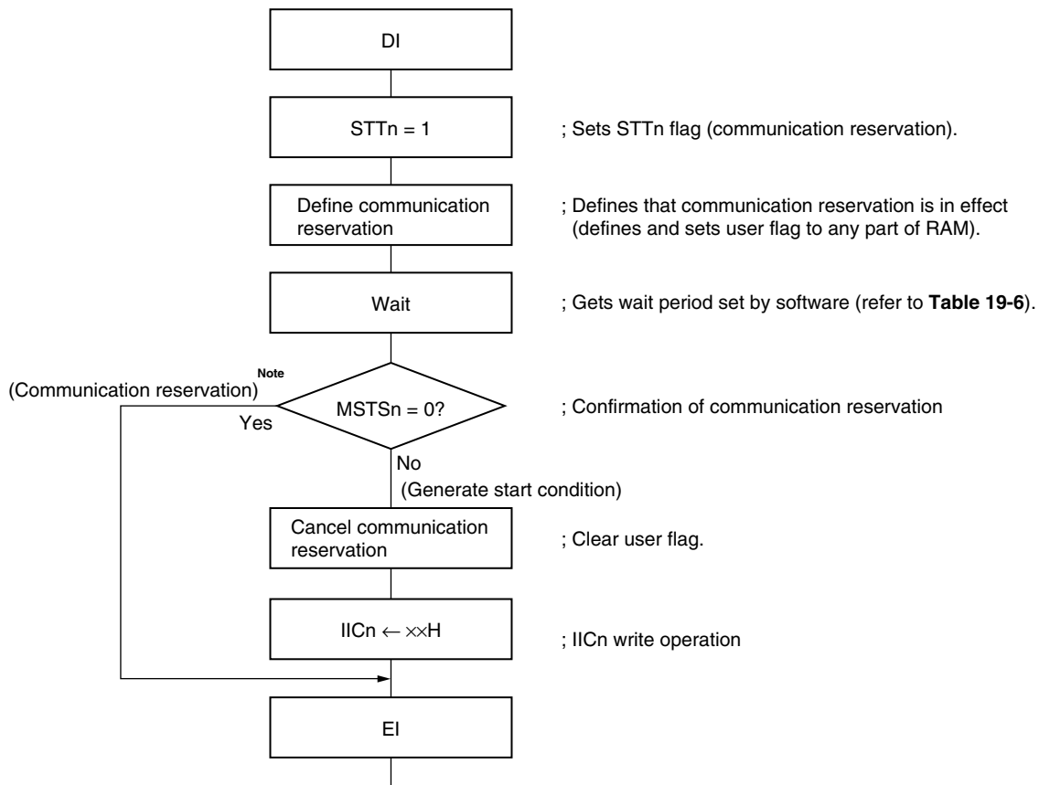
Figure 19-15. Communication Reservation Flowchart
