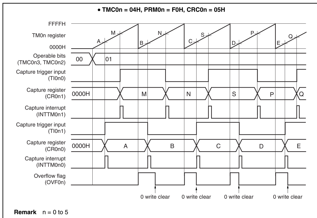
Figure 8-39. Timing Example of Pulse Width Measurement (1)
