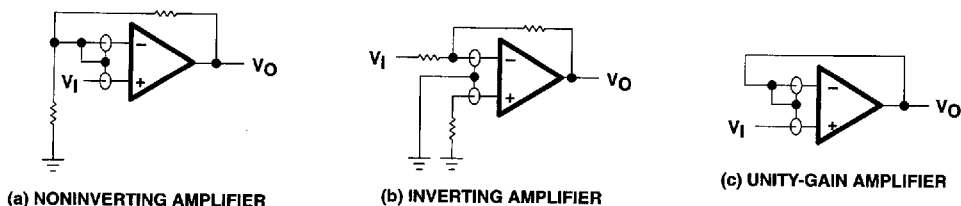
Figure 40. Guard-Ring Schemes
