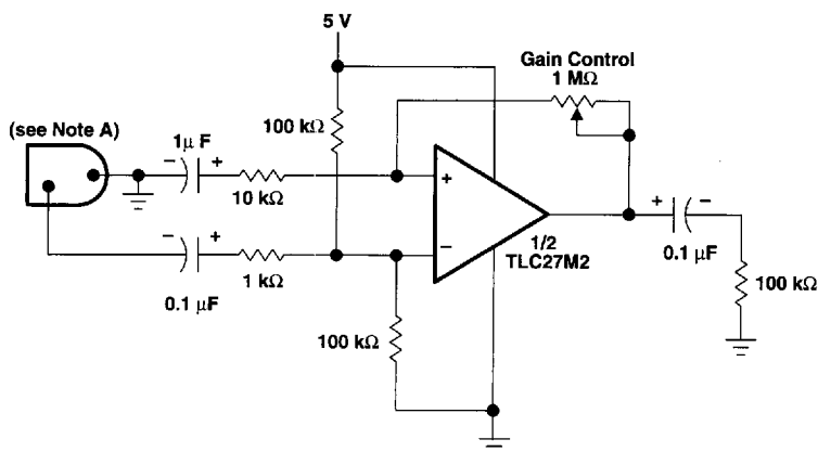
Figure 46. Microphone Preamplifier
