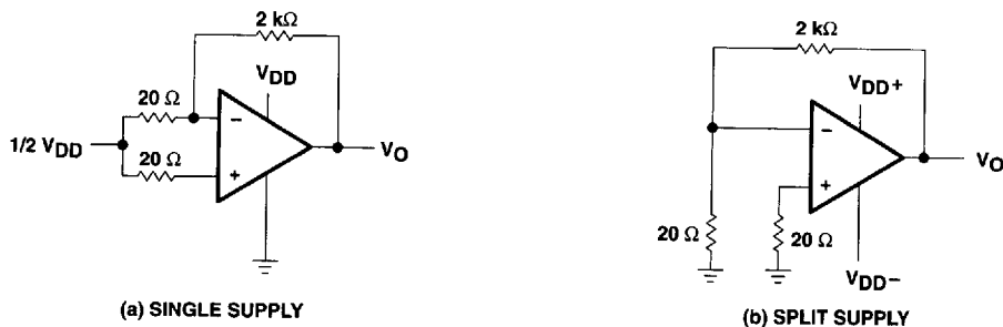
Figure 2. Noise-Test Circuit
