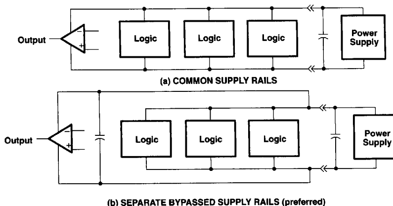
Figure 39. Common Versus Separate Supply Rails
