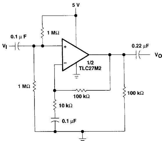
Figure 49. Single-Rail AC Amplifiers
