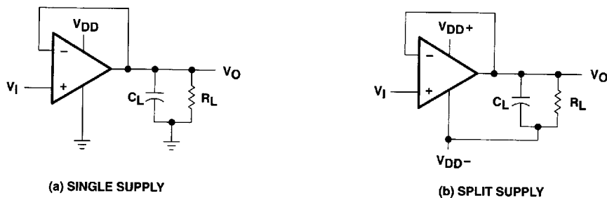
Figure 1. Unity-Gain Amplifier
