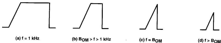
Figure 5. Full-Power-Response Output Signal
