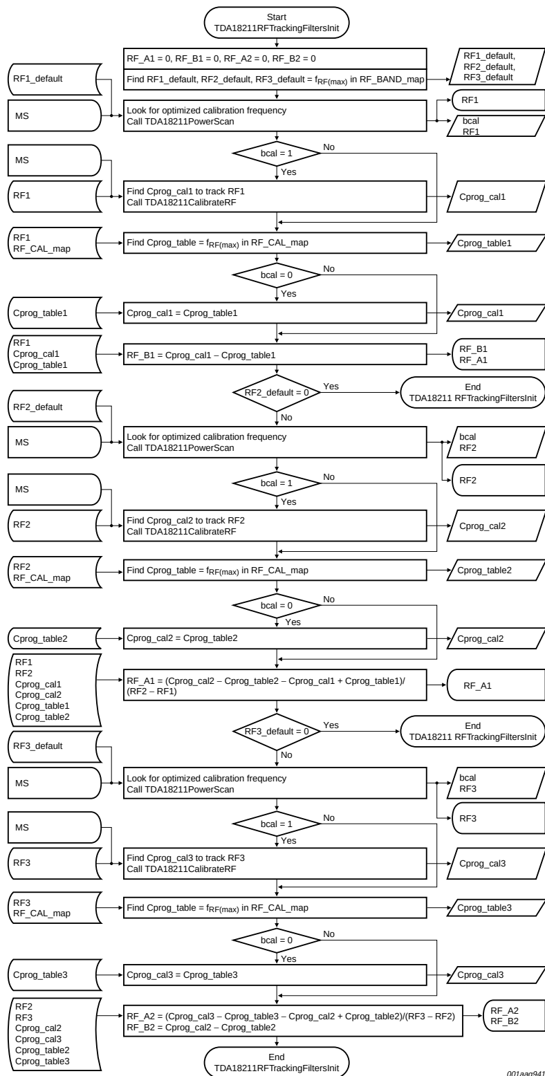
Fig 11. Flowchart TDA18211RFTrackingFiltersInit
