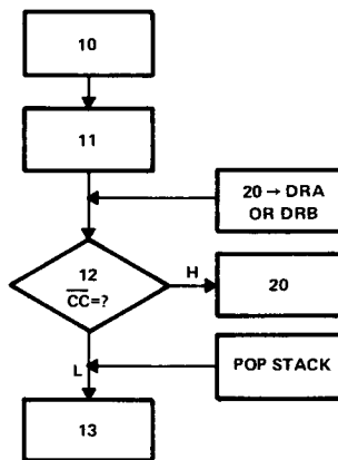
(p) CONDITIONAL BRANCH AND POP (DEC DISABLED)
