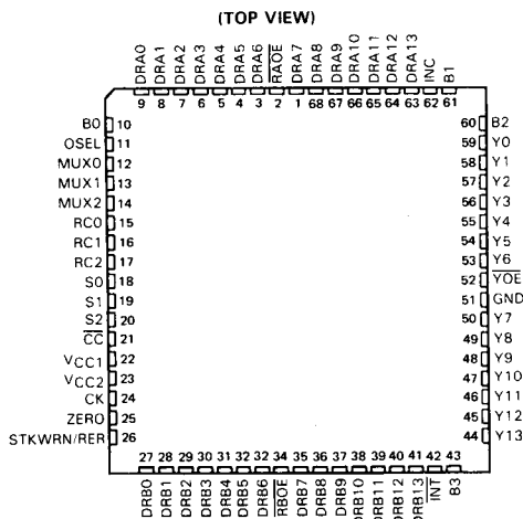
SN54AS890 . . . FD PACKAGE SN74AS890 . . . FN PACKAGE (TOP VIEW)
