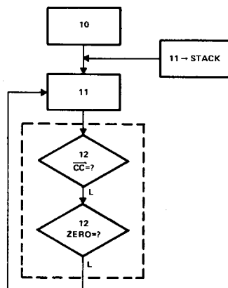
(f) REPEAT (CC FORCED, DEC DISABLED) 1
