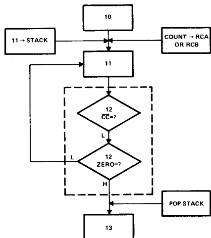
(e) CONDITIONAL LOOP ON STACK (CC FORCED, DEC ENABLED) 1
