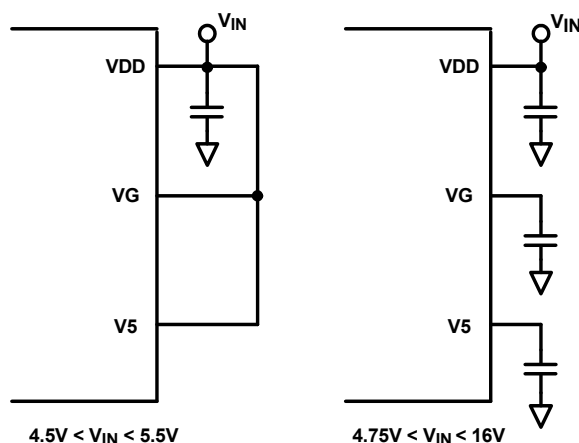
Figure 7. Supply Connections
