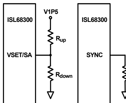
Figure 6. Pin-Strap Pins
