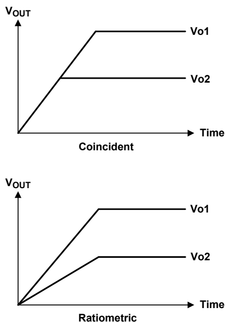
Figure 12. Tracking Modes
