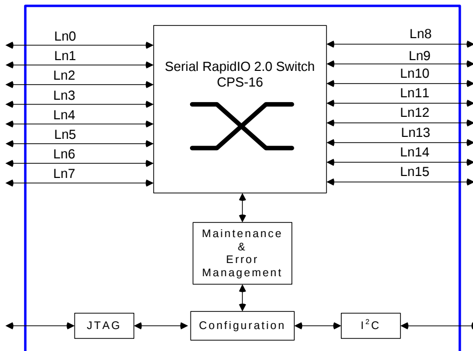
Figure 1 Block diagram
