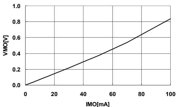
IMO VS. VMO VDD=5V T_a=25[^\circ\text{C}]
