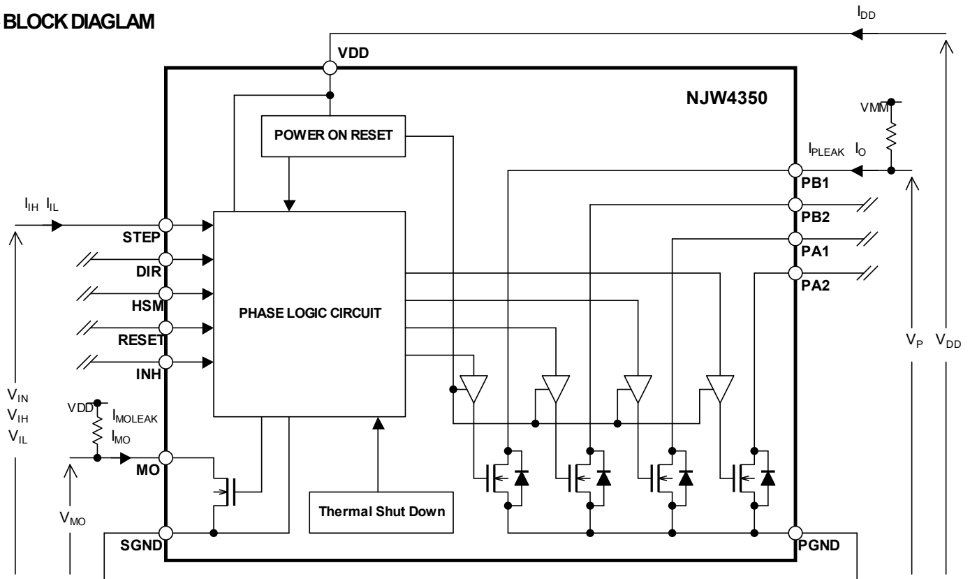
Fig.2 Brock Diagram
