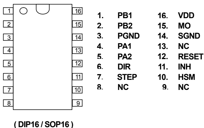
Fig.1 Pin Configuration
