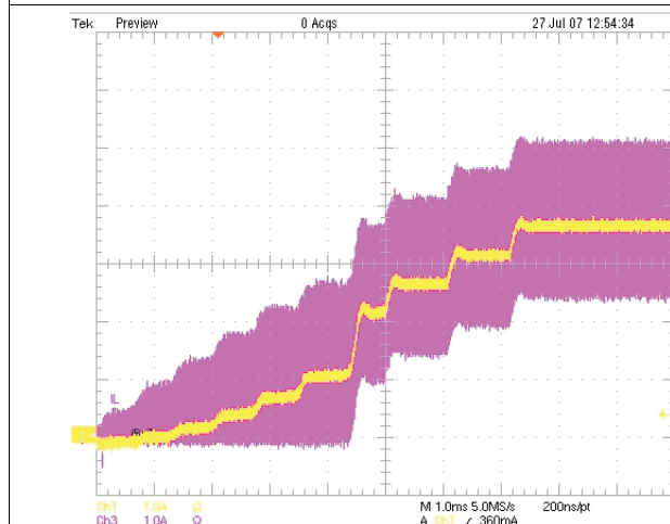
Figure 22. Inductor Current and Battery Current Soft-Start
