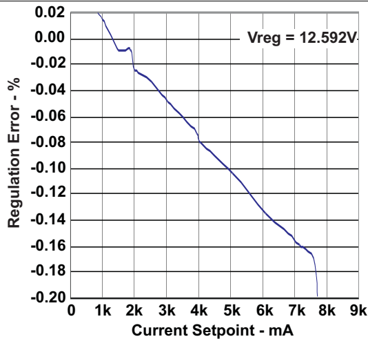
Figure 4. VFB Voltage Regulation Accuracy vs Charge Current
