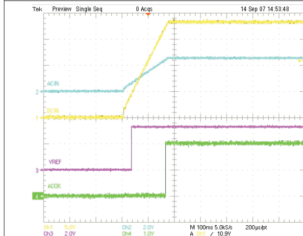
Figure 20. Charger When Adapter Inserted
