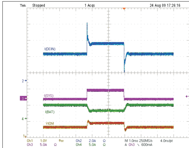
Figure 18. Transient System Load (DPM) Response: Charge Current Dropped From 4A to 2A
