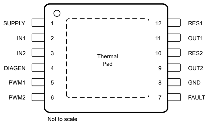
Figure 5-1. DGN Package 12-Pin HVSSOP With PowerPAD™ Integrated Circuit Package (Top View)
