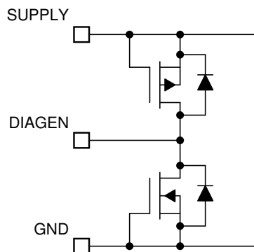
Figure 7-9. DIAGEN Pin
