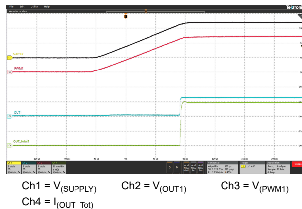
Figure 6-10. Power-Up Sequence
