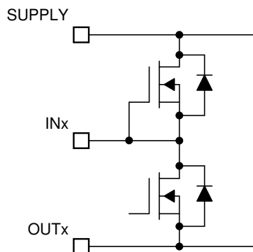
Figure 7-13. INx Pins
