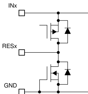
Figure 7-12. RESx Pins
