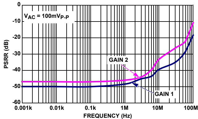
FIGURE 13. PSRR vs FREQUENCY
