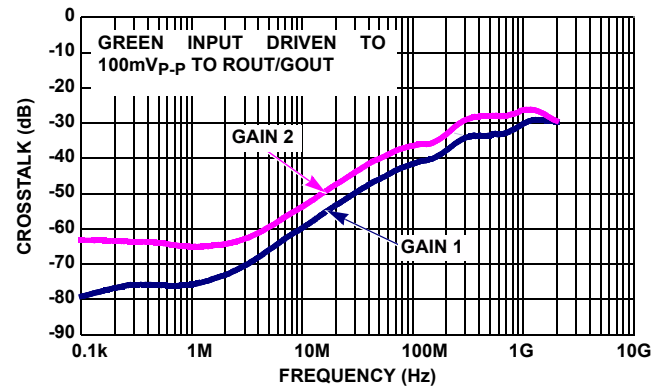
FIGURE 14. ACTIVE CHANNEL CROSSTALK
