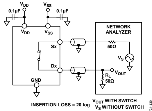
Figure 37. Insertion Loss/-3 dB Bandwidth
