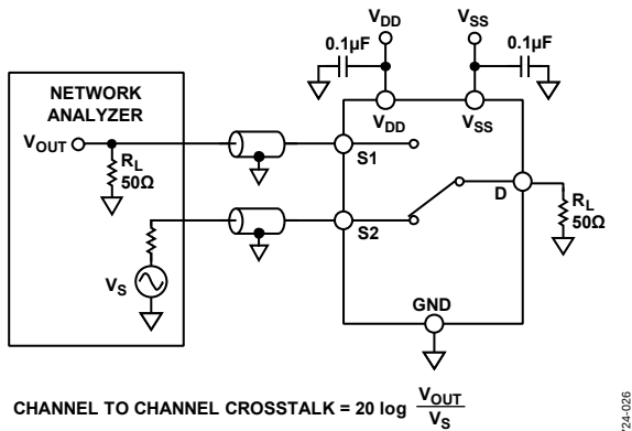
Figure 33. Channel to Channel Crosstalk
