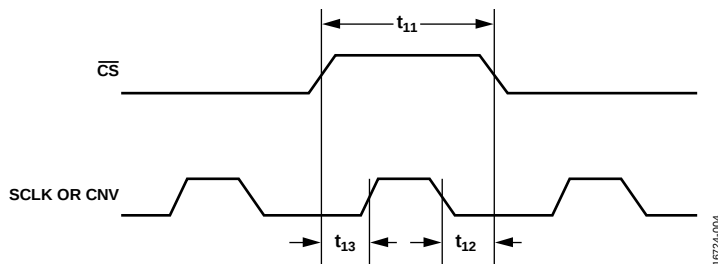
Figure 5. SCLK or CNV and \overline{CS} Timing Diagram
