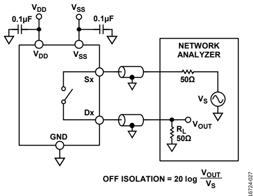
Figure 34. Off Isolation
