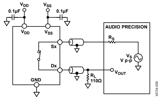
Figure 38. THD + N
