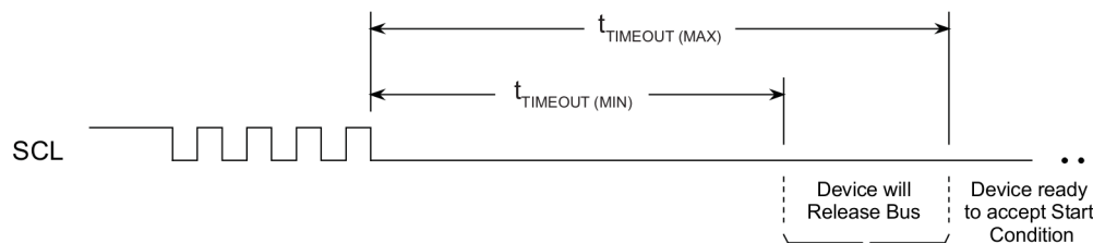
Figure 5-5. SMBus Timeout
