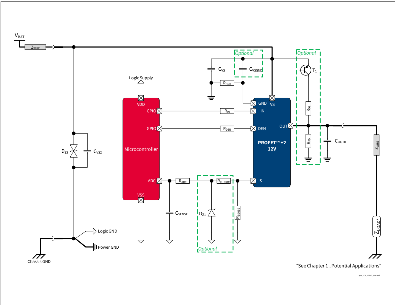
Figure 42 BTS7008-1EPZ Application Diagram
