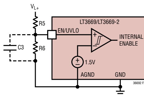
Figure 23. Undervoltage Lockout
