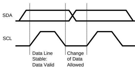
Figure 14. Bit Transfer
