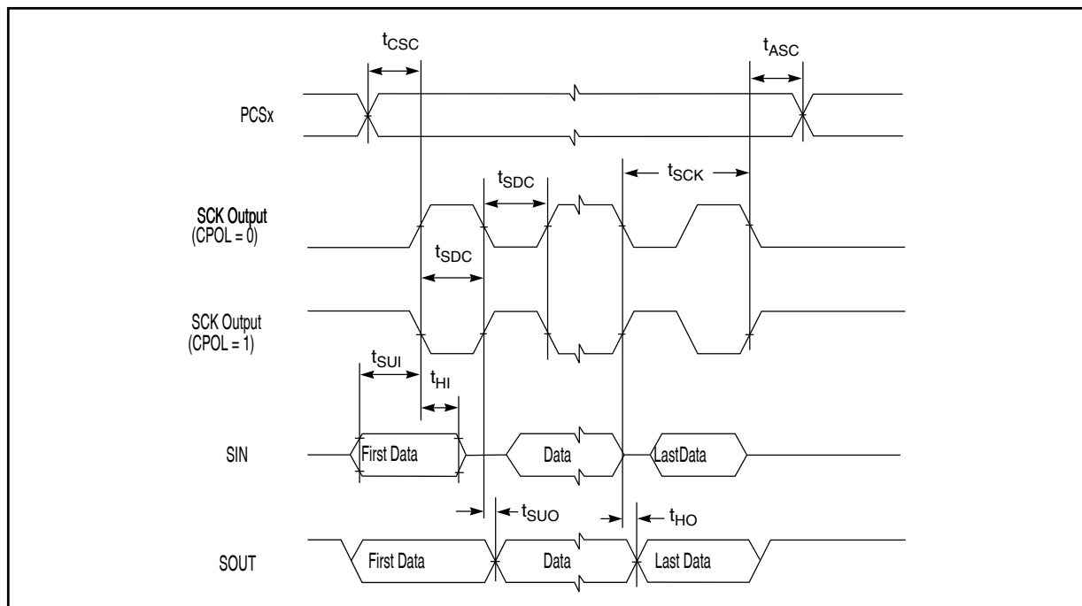
Figure 30. DSPI CMOS master mode – classic timing, CPHA = 0
