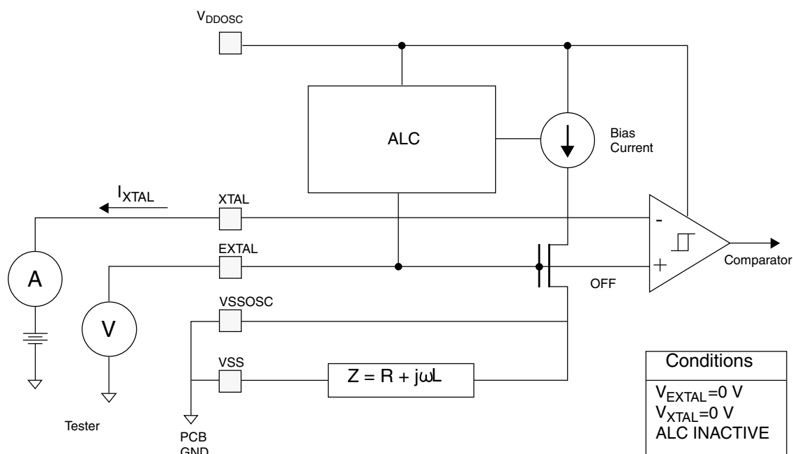
Figure 9. Test circuit
