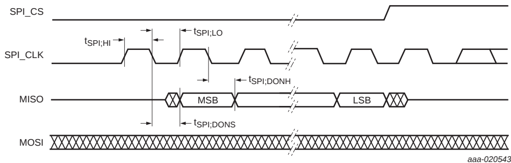
Fig 18. SPI read timing
