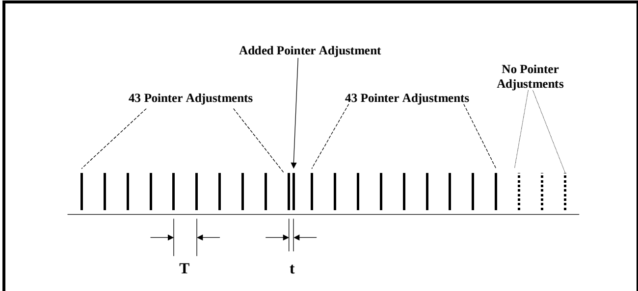
FIGURE 60. ILLUSTRATION OF THE 87-3 ADD POINTER ADJUSTMENT PATTERN
