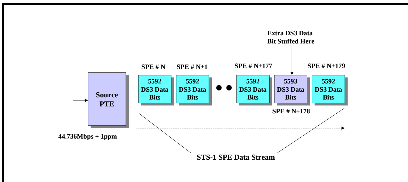
FIGURE 47. AN ILLUSTRATION OF THE STS-1 SPE TRAFFIC THAT WILL BE GENERATED BY THE "SOURCE" PTE, WHEN MAPPING IN A DS3 SIGNAL THAT HAS A BIT RATE OF 44.736\text{Mbps} + 1\text{PPM} , INTO AN STS-1 SIGNAL
