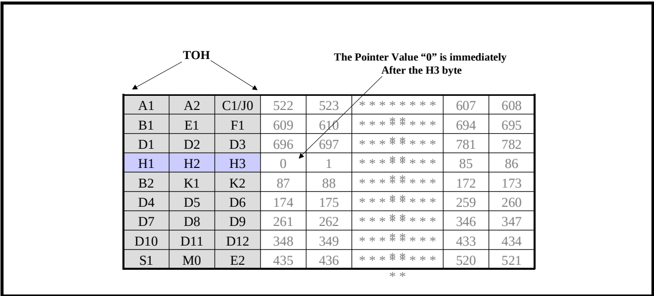
FIGURE 51. THE RELATIONSHIP BETWEEN THE CONTENTS OF THE "POINTER BITS" (E.G., THE 10-BIT EXPRESSION WITHIN THE H1 AND H2 BYTES) AND THE LOCATION OF THE J1 BYTE WITHIN THE ENVELOPE CAPACITY OF AN STS-1 FRAME
