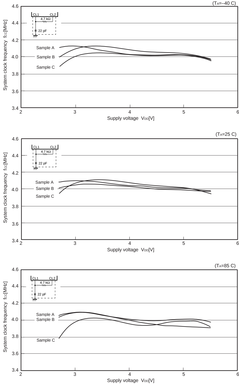
f cc vs V DD (RC Oscillation, R = 4.7 kΩ, C = 22 pF)
