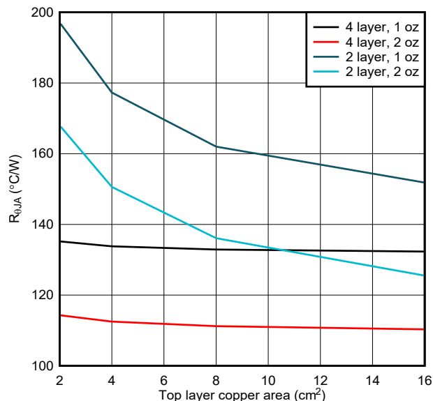
Figure 9-33. SOT, PCB junction-to-ambient thermal resistance vs copper area
