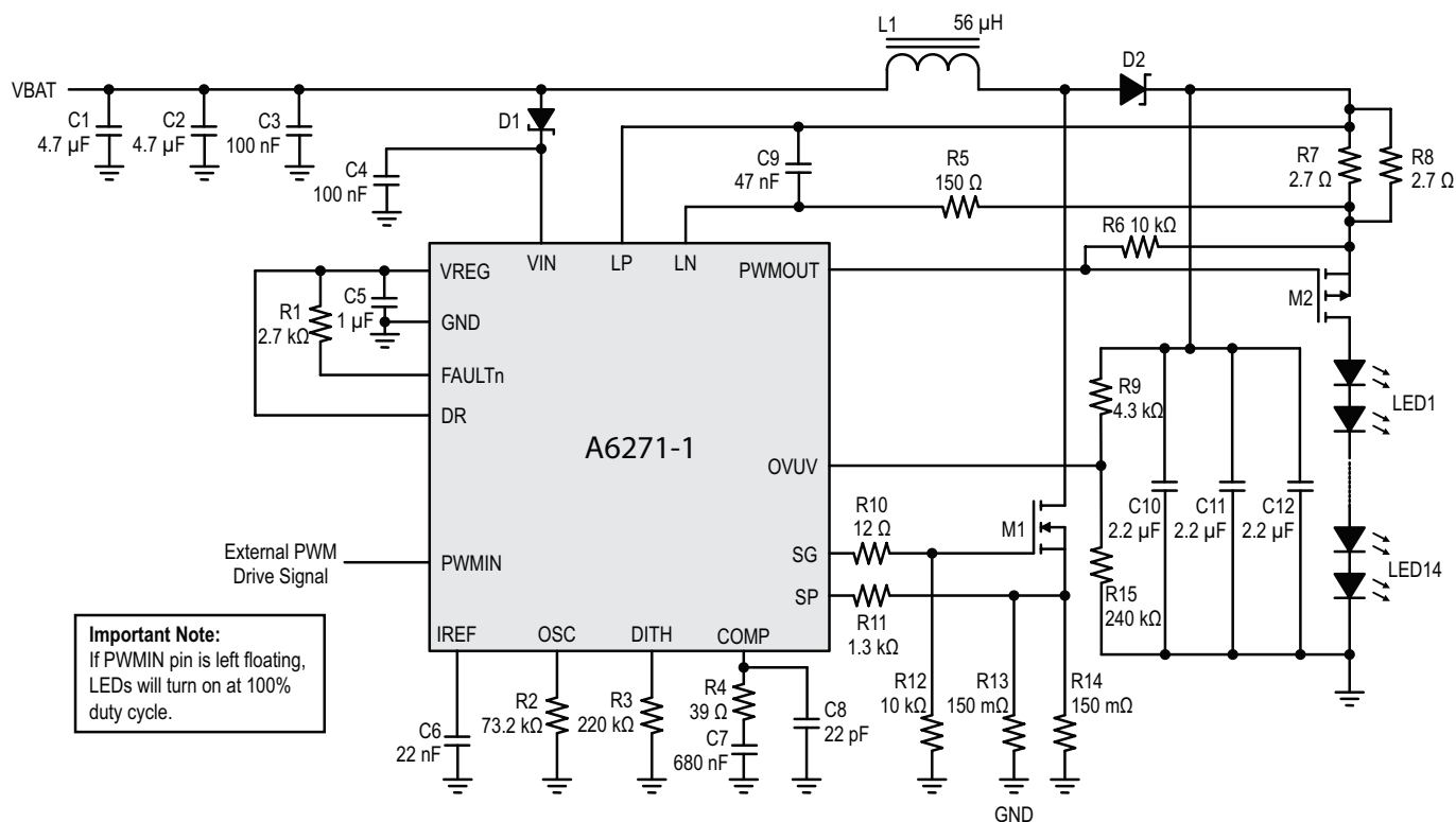
Figure 12: Boost Driving 14 LEDs at 150 mA, Switching Frequency 350 kHz
