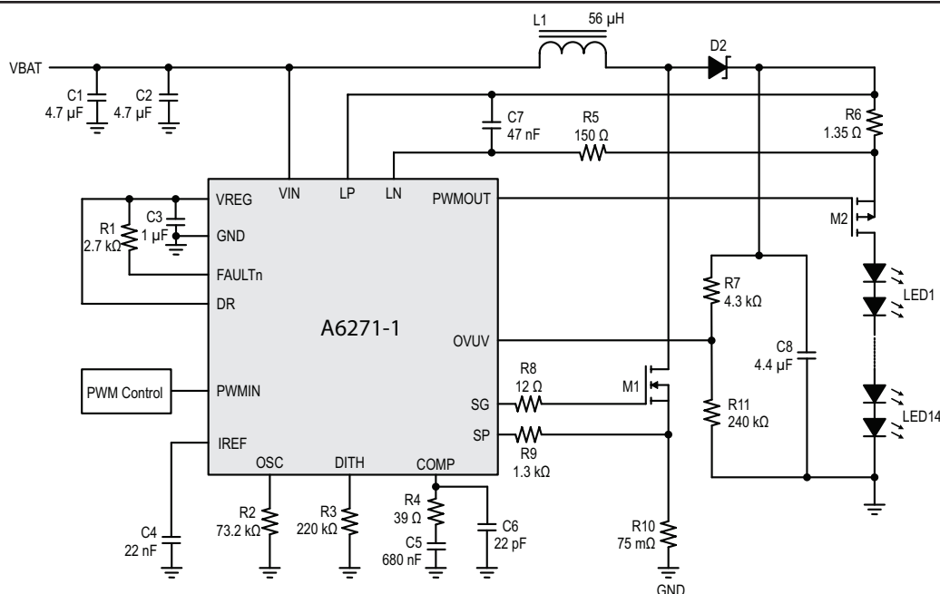
Figure 1: Boost Switcher Driving 14 LEDs at 150 mA
