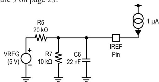
Figure 3: Charging Of Soft-Start Cap During Power Up
