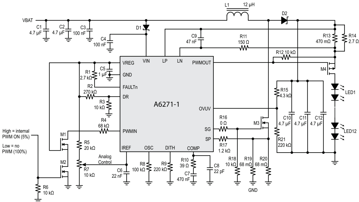
Figure 11: Boost Driving 12 LEDs at 500 mA, Switching Frequency 250 kHz
