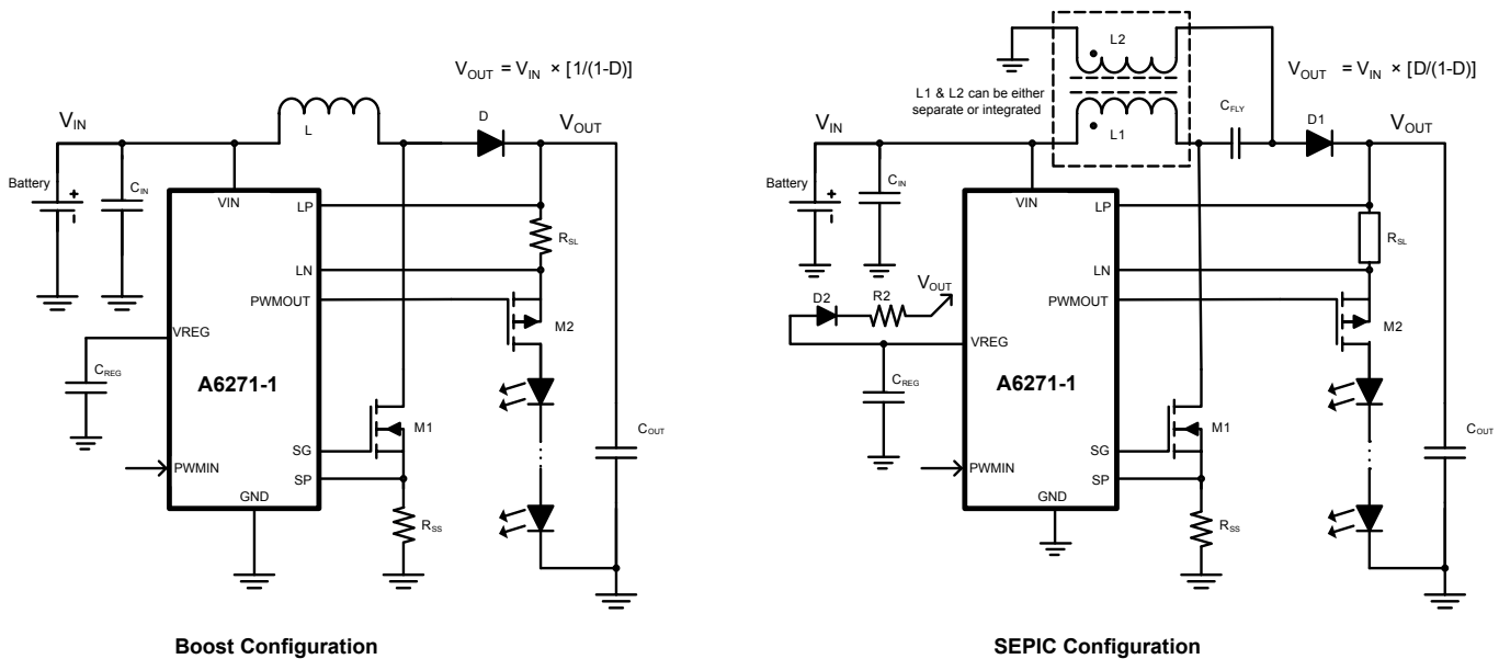
Figure A-1: Comparison of A6271-1 in Boost and SEPIC configurations
