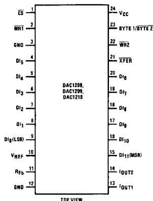
Dual-In-Line Package
