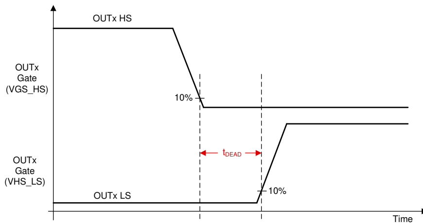
Figure 8-19. Dead Time
