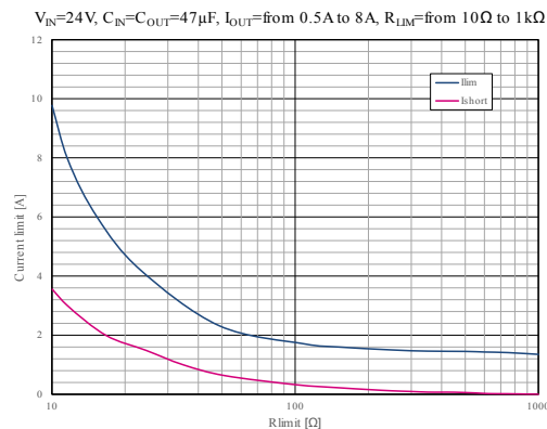
Figure 7. Current limit vs. R_{\text{limit}}
