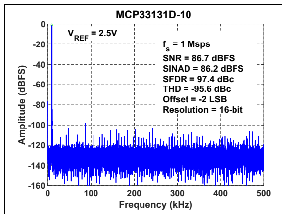
FIGURE 2-11: FFT for 10 kHz Input Signal: f_S = 1\text{ Msp} , V_{IN} = -1\text{ dBFS} , V_{REF} = 2.5\text{V} .
