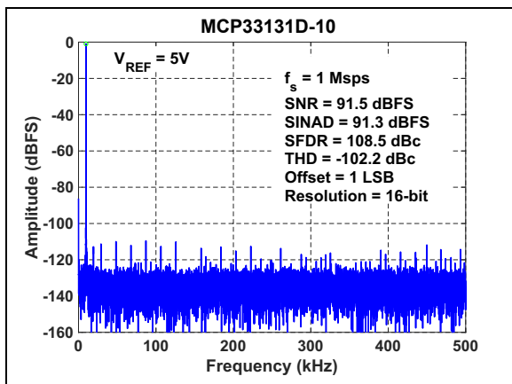
FIGURE 2-8: FFT for 10 kHz Input Signal: f_S = 1\text{ Msp} , V_{IN} = -1\text{ dBFS} , V_{REF} = 5\text{V} .
